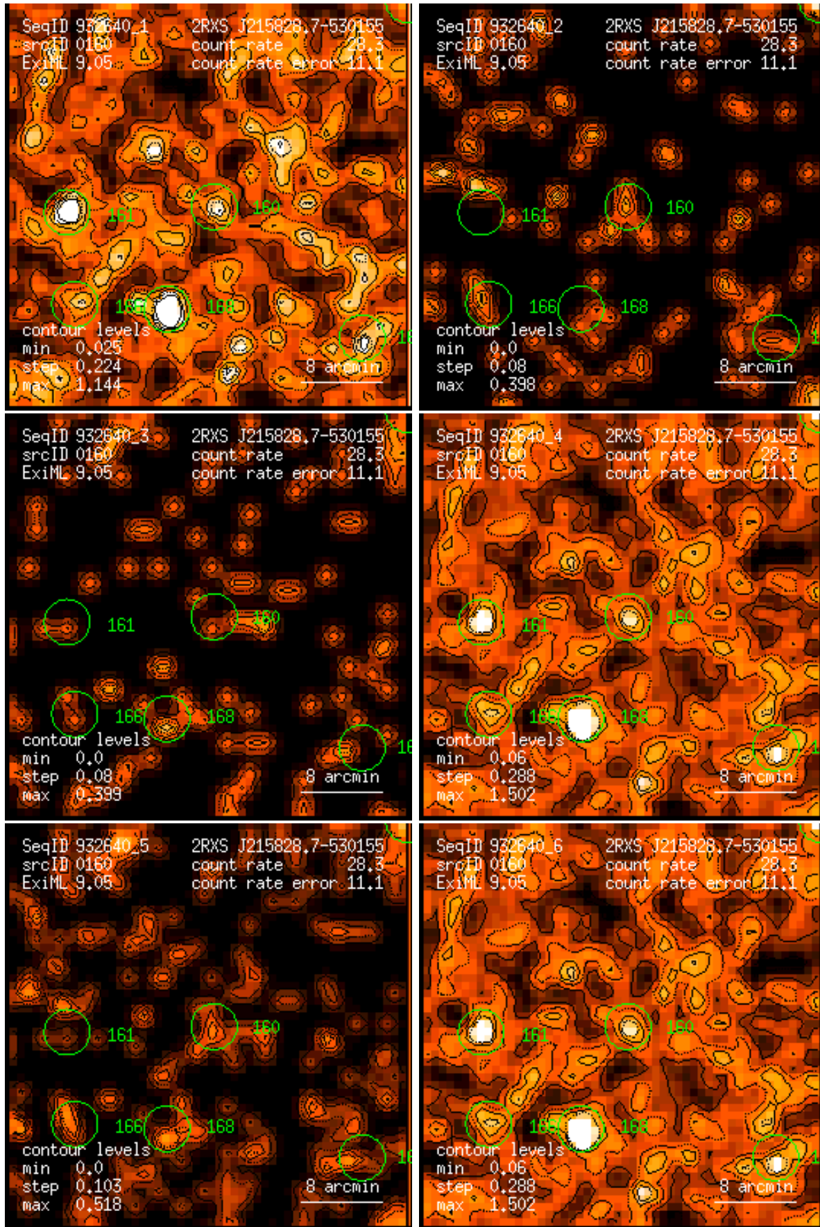
Figure 160: RASS 932640: detection 0160: band rate images, Gaussian filter: (1) PSPC channels 11 – 41, (2) 52 – 90, (3) 91 – 201, (4) 11 – 235, (5) 52 – 201, (6) 11 – 201. Broad band rates in counts/ks. Band rate contour levels in counts/ks/arcmin 2 .
