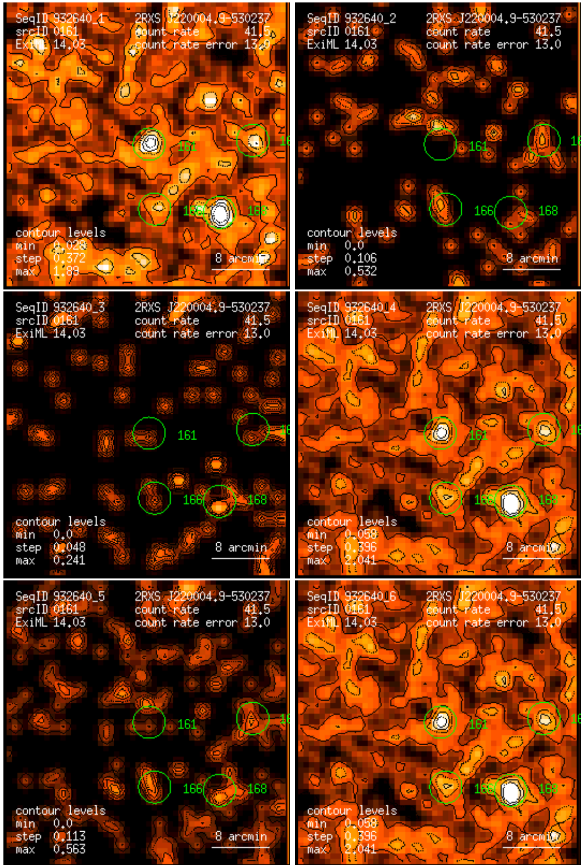
Figure 161: RASS 932640: detection 0161: band rate images, Gaussian filter: (1) PSPC channels 11 – 41, (2) 52 – 90, (3) 91 – 201, (4) 11 – 235, (5) 52 – 201, (6) 11 – 201. Broad band rates in counts/ks. Band rate contour levels in counts/ks/arcmin 2 .
