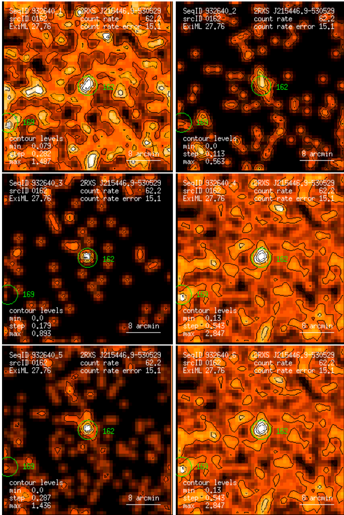
Figure 162: RASS 932640: detection 0162: band rate images, Gaussian filter: (1) PSPC channels 11 – 41, (2) 52 – 90, (3) 91 – 201, (4) 11 – 235, (5) 52 – 201, (6) 11 – 201. Broad band rates in counts/ks. Band rate contour levels in counts/ks/arcmin 2 .
