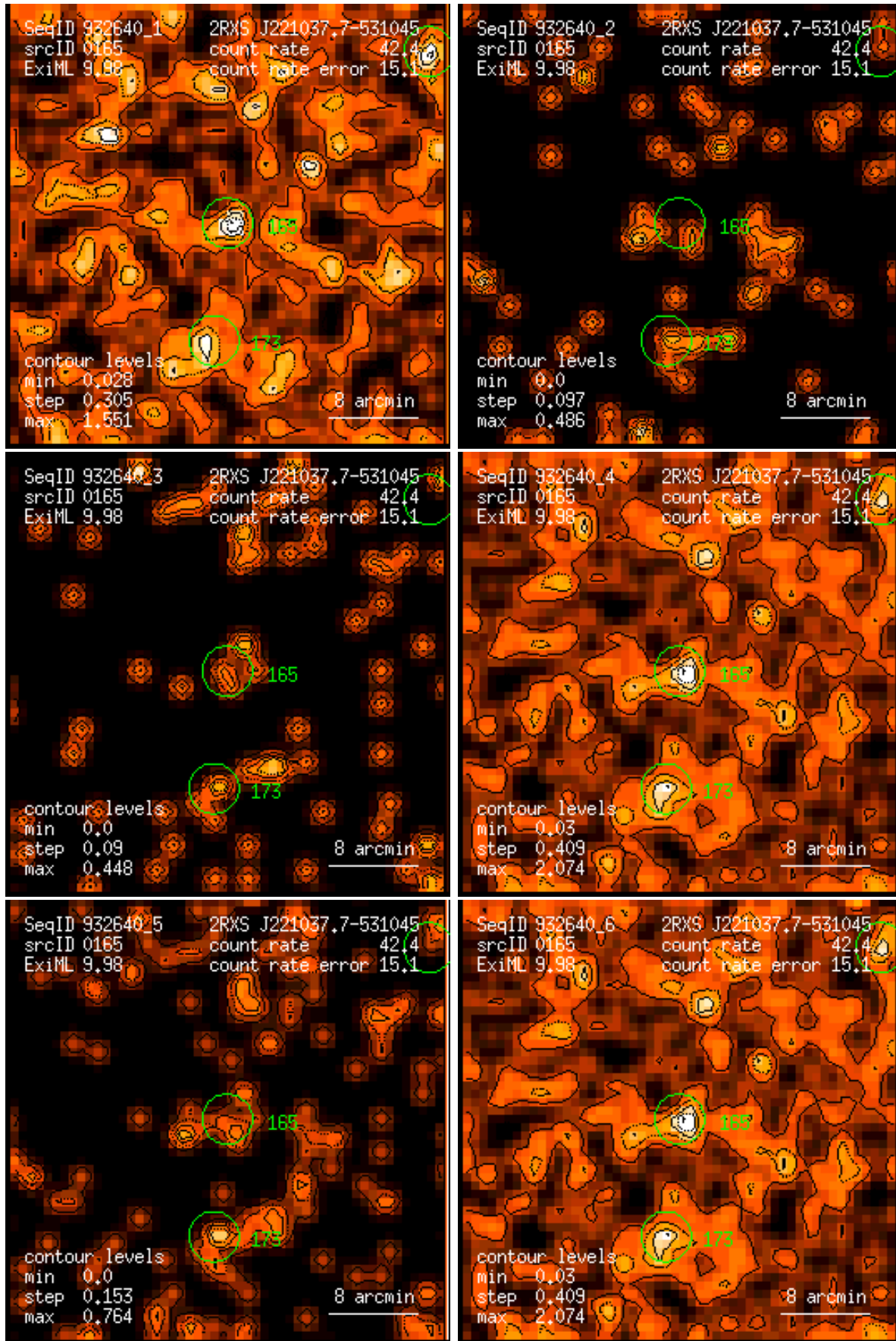
Figure 165: RASS 932640: detection 0165: band rate images, Gaussian filter: (1) PSPC channels 11 – 41, (2) 52 – 90, (3) 91 – 201, (4) 11 – 235, (5) 52 – 201, (6) 11 – 201. Broad band rates in counts/ks. Band rate contour levels in counts/ks/arcmin 2 .
