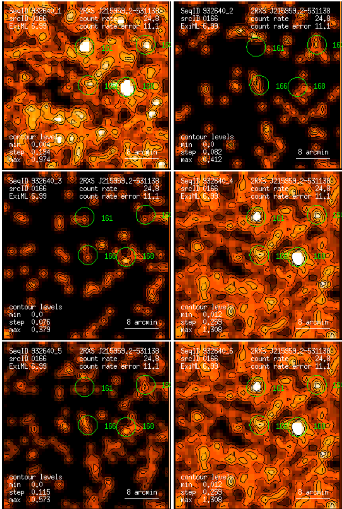
Figure 166: RASS 932640: detection 0166: band rate images, Gaussian filter: (1) PSPC channels 11 – 41, (2) 52 – 90, (3) 91 – 201, (4) 11 – 235, (5) 52 – 201, (6) 11 – 201. Broad band rates in counts/ks. Band rate contour levels in counts/ks/arcmin 2 .
