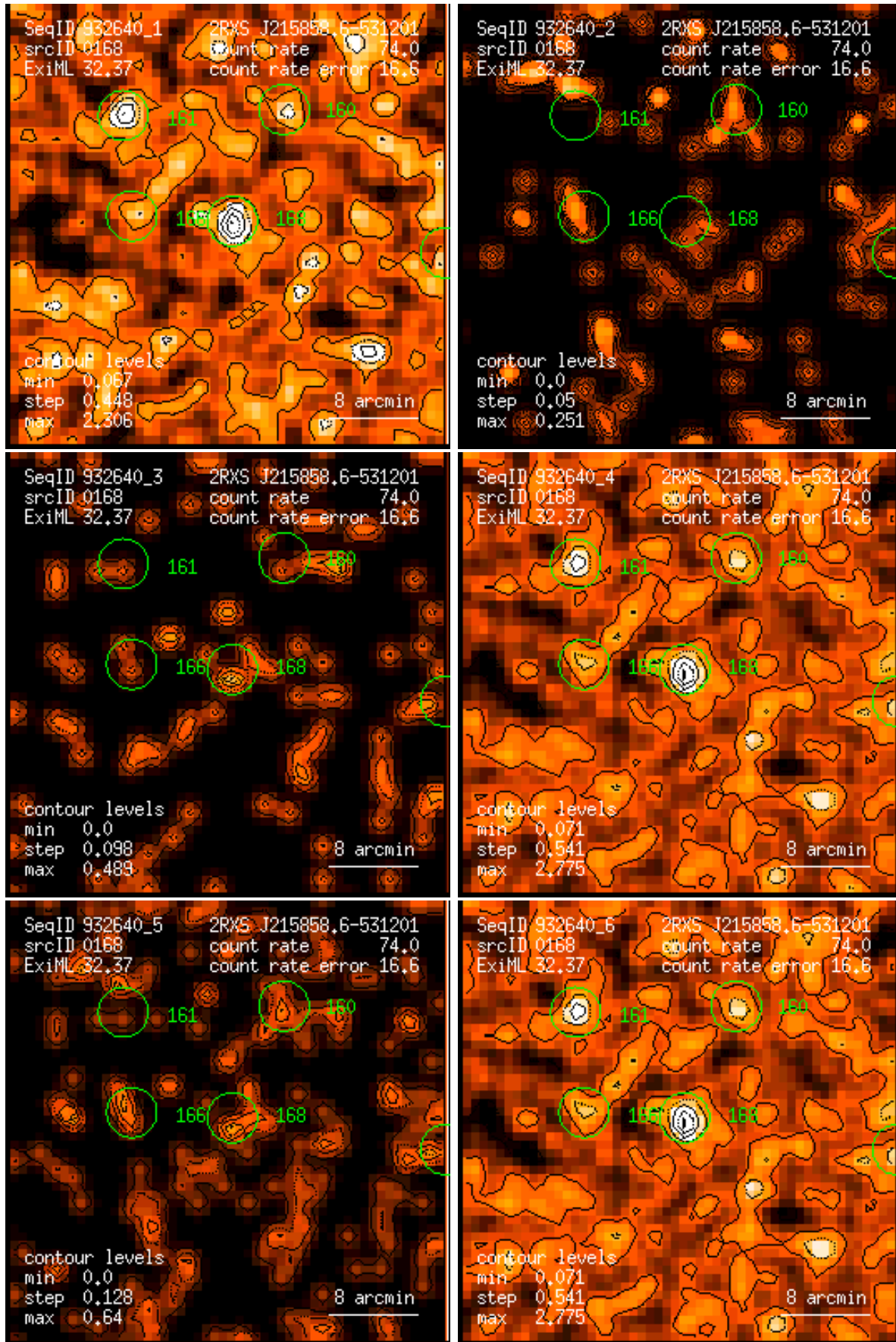
Figure 168: RASS 932640: detection 0168: band rate images, Gaussian filter: (1) PSPC channels 11 – 41, (2) 52 – 90, (3) 91 – 201, (4) 11 – 235, (5) 52 – 201, (6) 11 – 201. Broad band rates in counts/ks. Band rate contour levels in counts/ks/arcmin 2 .
