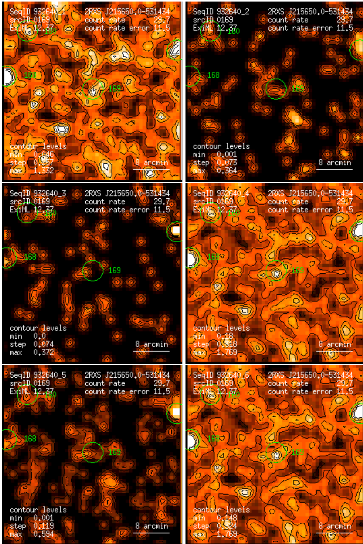
Figure 169: RASS 932640: detection 0169: band rate images, Gaussian filter: (1) PSPC channels 11 – 41, (2) 52 – 90, (3) 91 – 201, (4) 11 – 235, (5) 52 – 201, (6) 11 – 201. Broad band rates in counts/ks. Band rate contour levels in counts/ks/arcmin 2 .
