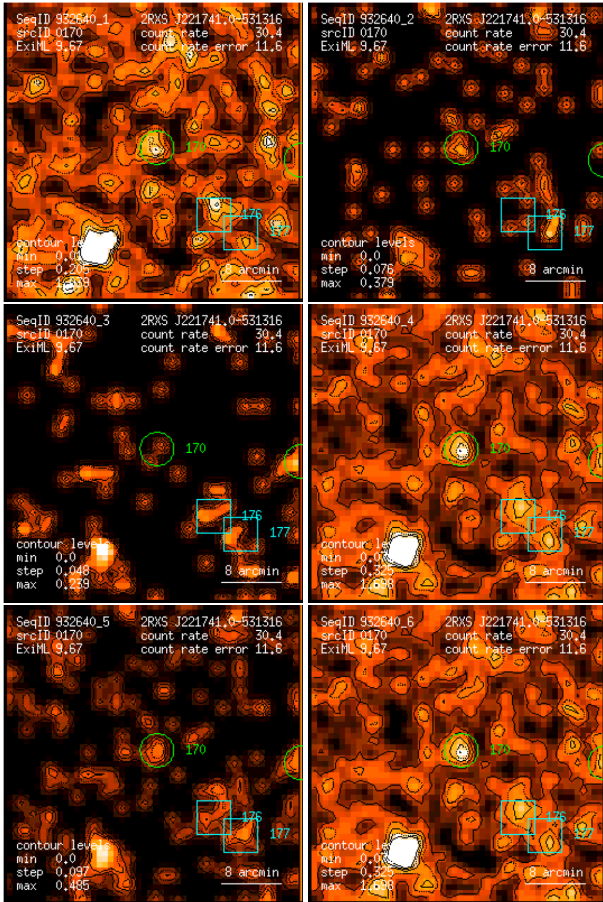
Figure 170: RASS 932640: detection 0170: band rate images, Gaussian filter: (1) PSPC channels 11 – 41, (2) 52 – 90, (3) 91 – 201, (4) 11 – 235, (5) 52 – 201, (6) 11 – 201. Broad band rates in counts/ks. Band rate contour levels in counts/ks/arcmin 2 .
