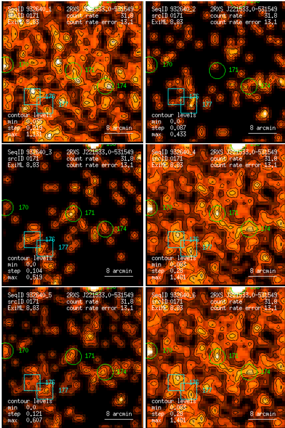
Figure 171: RASS 932640: detection 0171: band rate images, Gaussian filter: (1) PSPC channels 11 – 41, (2) 52 – 90, (3) 91 – 201, (4) 11 – 235, (5) 52 – 201, (6) 11 – 201. Broad band rates in counts/ks. Band rate contour levels in counts/ks/arcmin 2 .
