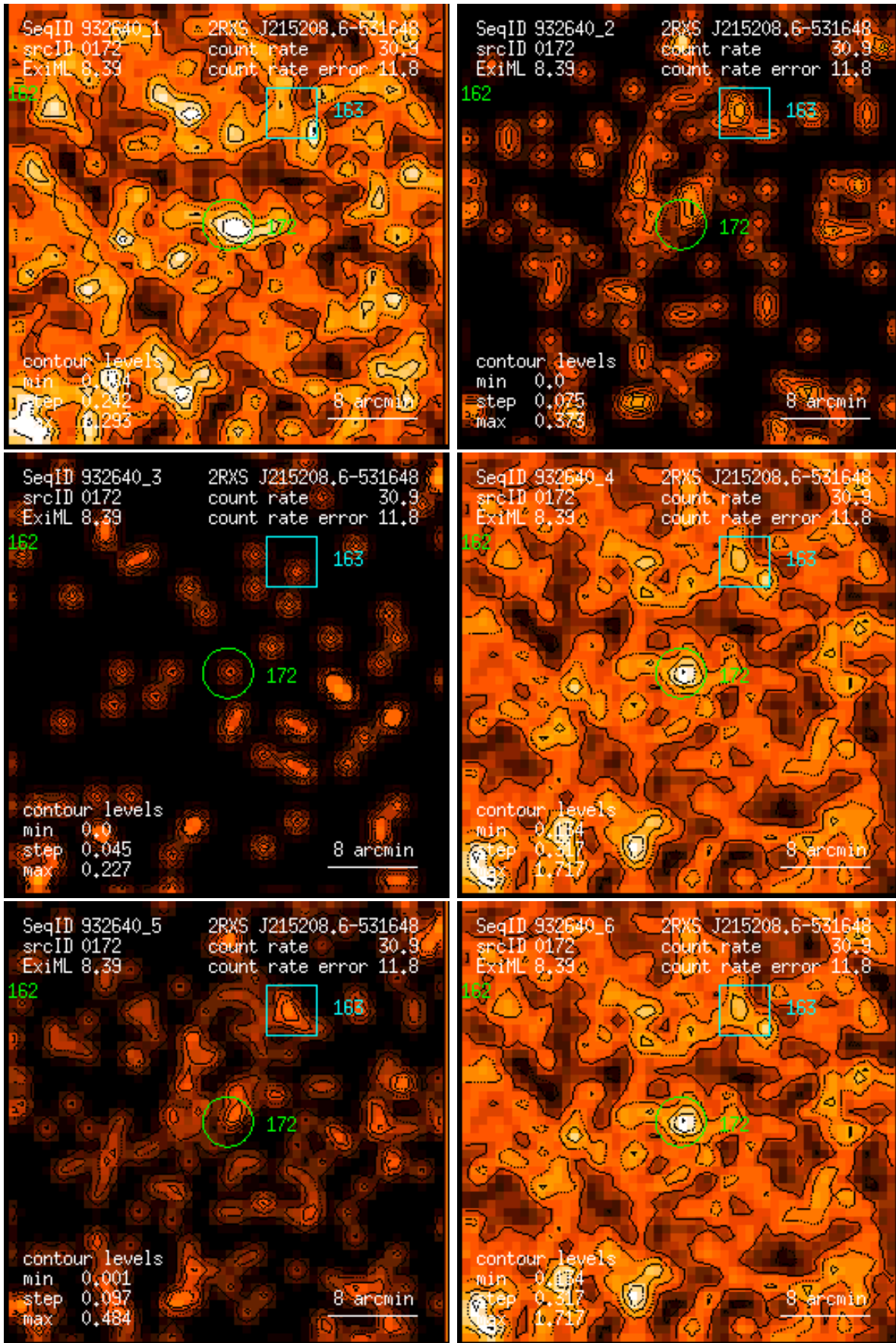
Figure 172: RASS 932640: detection 0172: band rate images, Gaussian filter: (1) PSPC channels 11 – 41, (2) 52 – 90, (3) 91 – 201, (4) 11 – 235, (5) 52 – 201, (6) 11 – 201. Broad band rates in counts/ks. Band rate contour levels in counts/ks/arcmin 2 .
