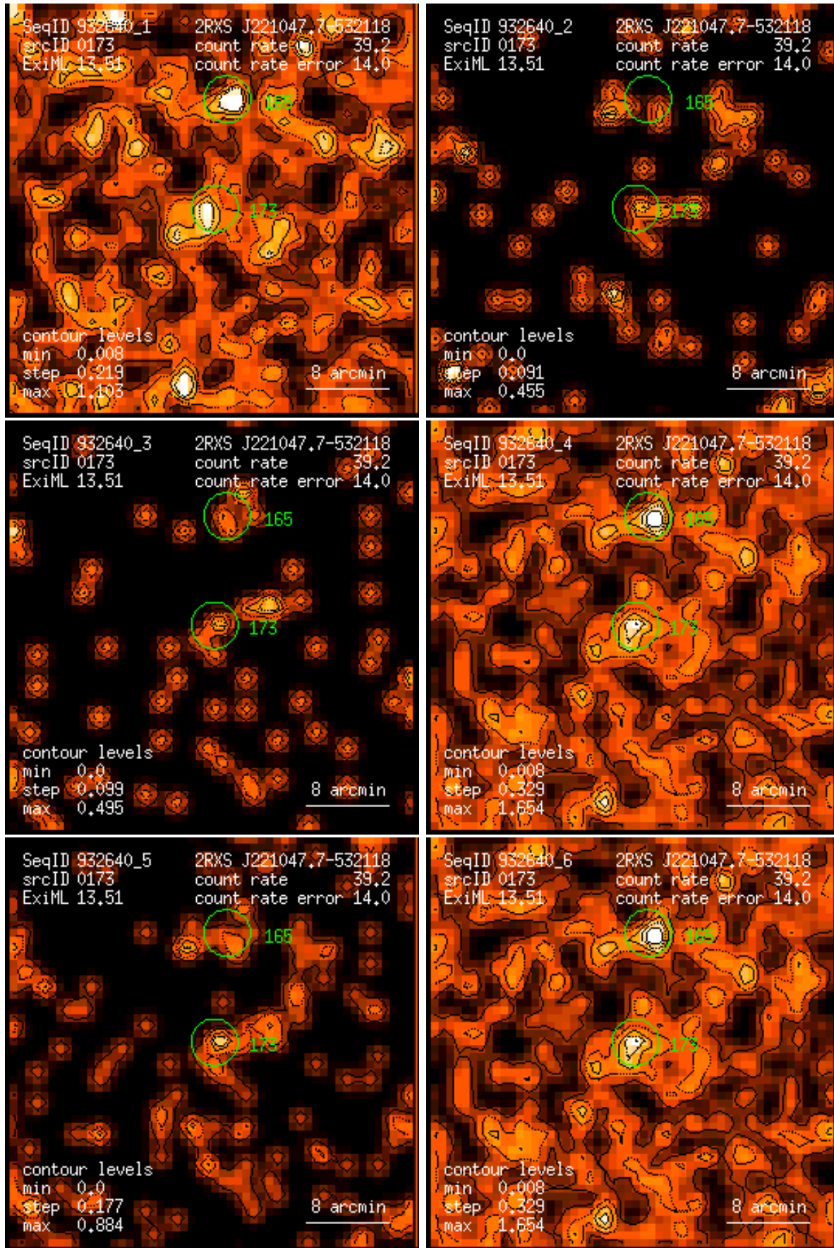
Figure 173: RASS 932640: detection 0173: band rate images, Gaussian filter: (1) PSPC channels 11 – 41, (2) 52 – 90, (3) 91 – 201, (4) 11 – 235, (5) 52 – 201, (6) 11 – 201. Broad band rates in counts/ks. Band rate contour levels in counts/ks/arcmin 2 .
