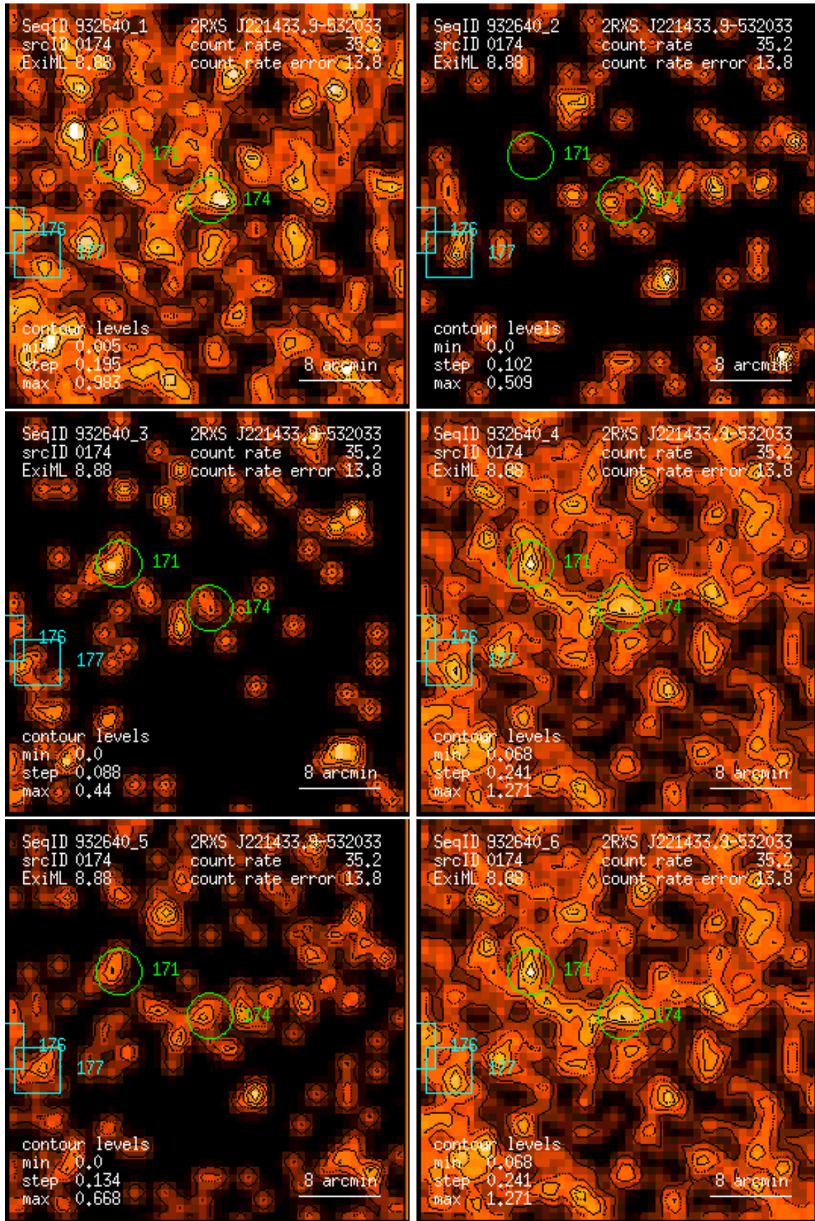
Figure 174: RASS 932640: detection 0174: band rate images, Gaussian filter: (1) PSPC channels 11 – 41, (2) 52 – 90, (3) 91 – 201, (4) 11 – 235, (5) 52 – 201, (6) 11 – 201. Broad band rates in counts/ks. Band rate contour levels in counts/ks/arcmin 2 .
