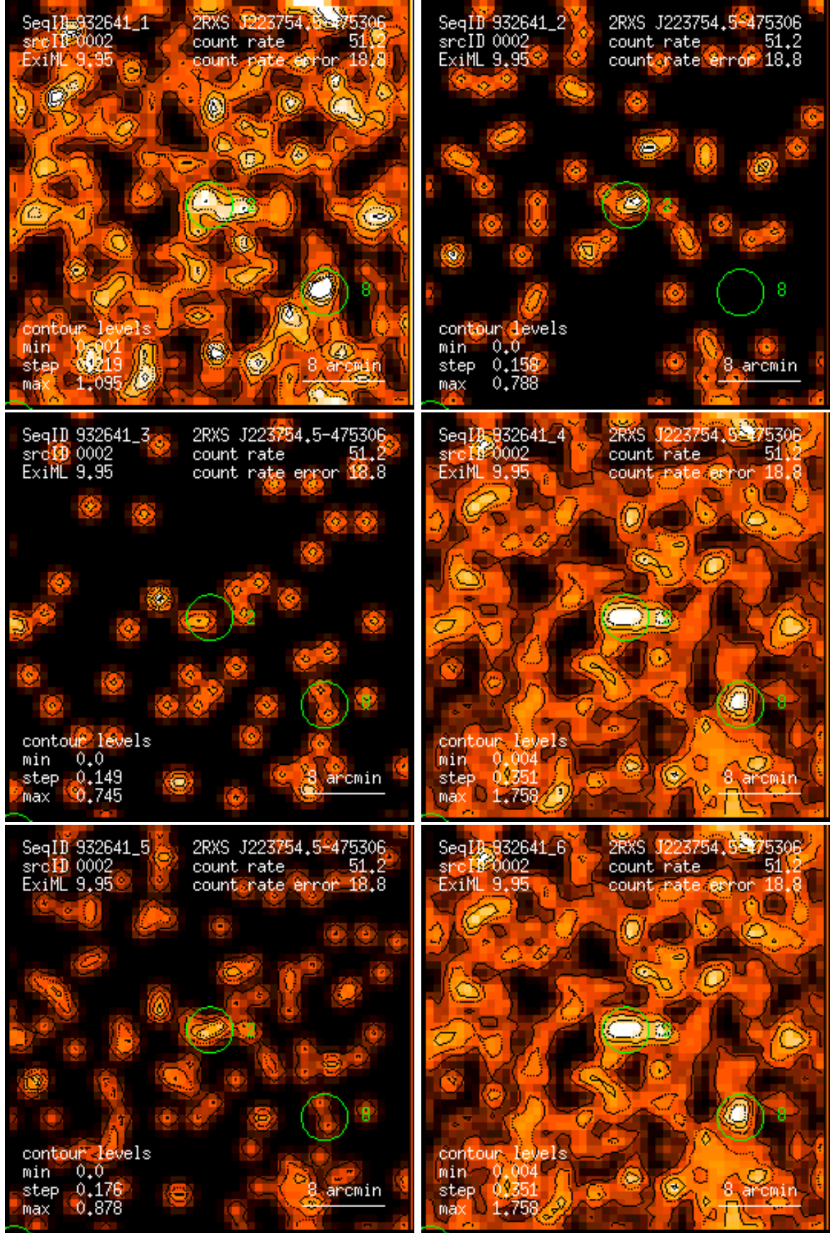
Figure 2: RASS 932641: detection 0002: band rate images, Gaussian filter: (1) PSPC channels 11 – 41, (2) 52 – 90, (3) 91 – 201, (4) 11 – 235, (5) 52 – 201, (6) 11 – 201. Broad band rates in counts/ks. Band rate contour levels in counts/ks/arcmin 2 .
