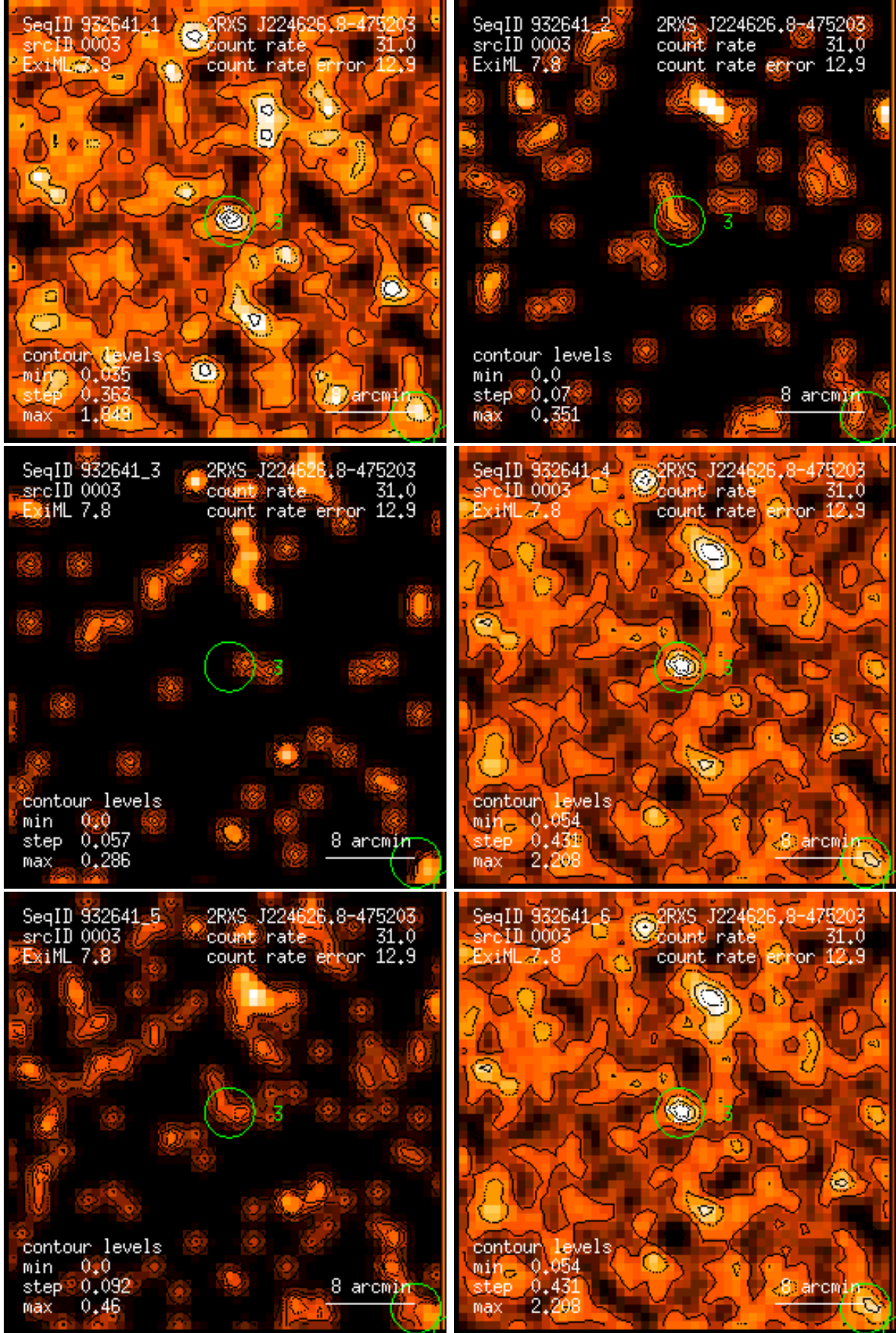
Figure 3: RASS 932641: detection 0003: band rate images, Gaussian filter: (1) PSPC channels 11 – 41, (2) 52 – 90, (3) 91 – 201, (4) 11 – 235, (5) 52 – 201, (6) 11 – 201. Broad band rates in counts/ks. Band rate contour levels in counts/ks/arcmin 2 .
