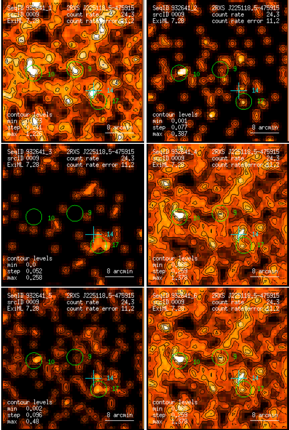
Figure 9: RASS 932641: detection 0009: band rate images, Gaussian filter: (1) PSPC channels 11 – 41, (2) 52 – 90, (3) 91 – 201, (4) 11 – 235, (5) 52 – 201, (6) 11 – 201. Broad band rates in counts/ks. Band rate contour levels in counts/ks/arcmin 2 .
