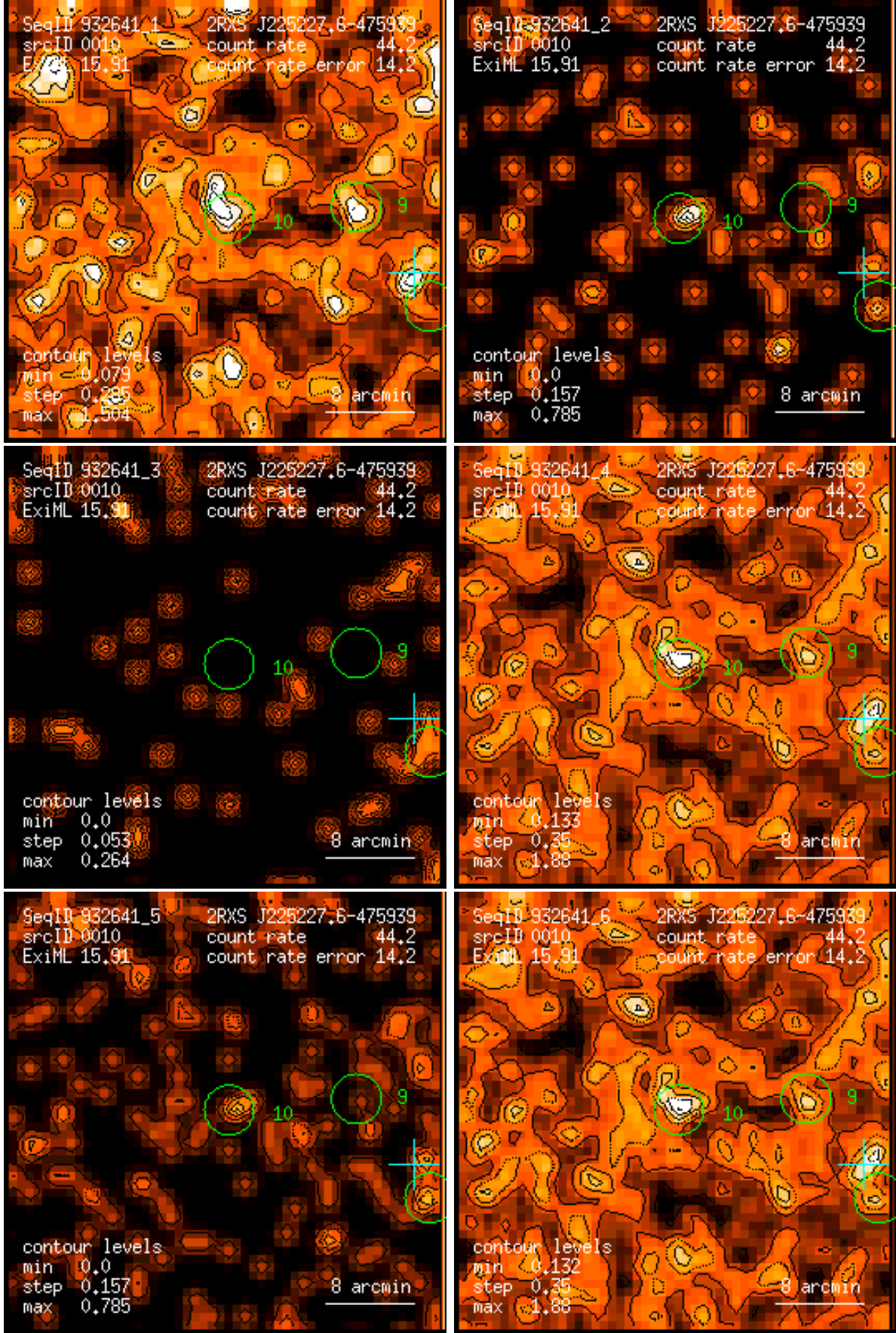
Figure 10: RASS 932641: detection 0010: band rate images, Gaussian filter: (1) PSPC channels 11 – 41, (2) 52 – 90, (3) 91 – 201, (4) 11 – 235, (5) 52 – 201, (6) 11 – 201. Broad band rates in counts/ks. Band rate contour levels in counts/ks/arcmin 2 .
