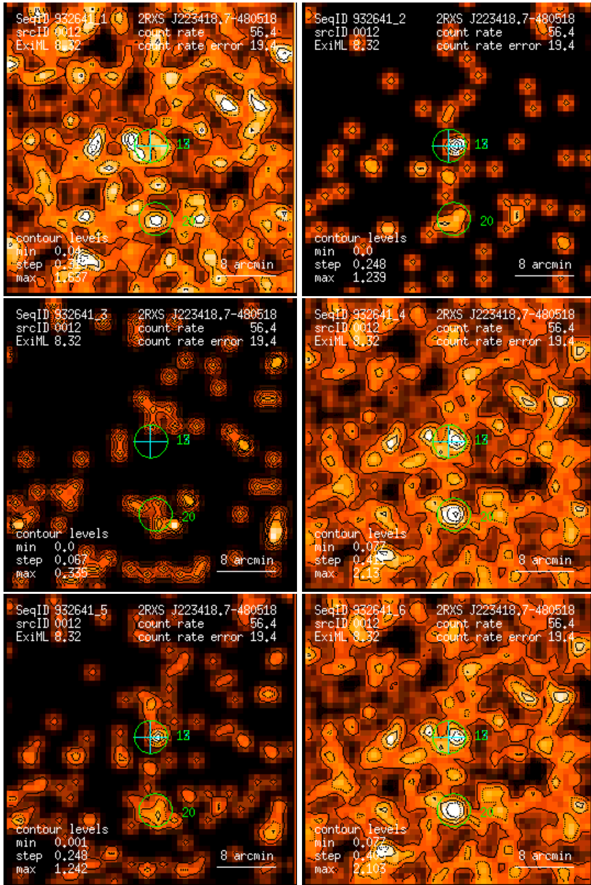
Figure 12: RASS 932641: detection 0012: band rate images, Gaussian filter: (1) PSPC channels 11 – 41, (2) 52 – 90, (3) 91 – 201, (4) 11 – 235, (5) 52 – 201, (6) 11 – 201. Broad band rates in counts/ks. Band rate contour levels in counts/ks/arcmin 2 .
