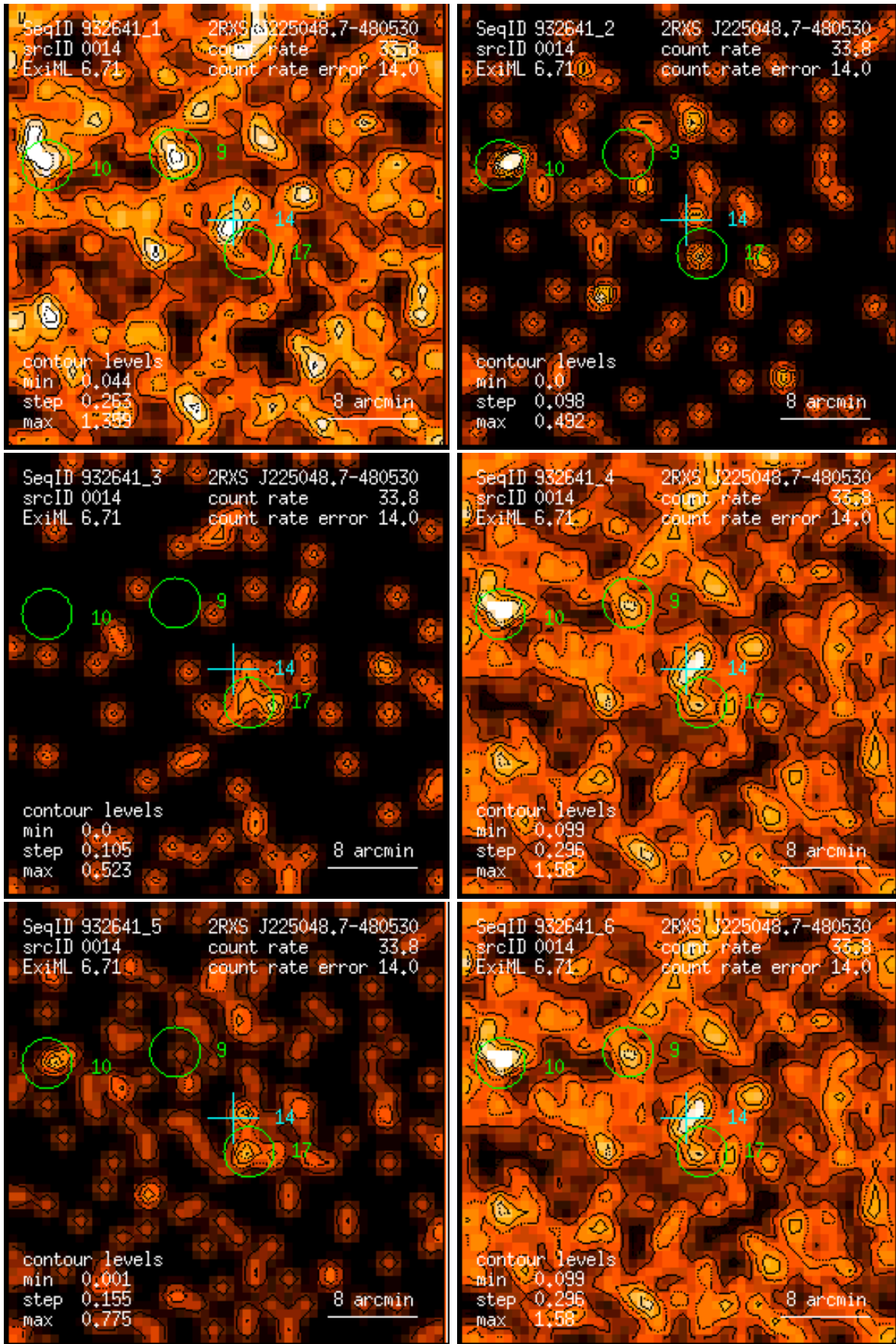
Figure 14: RASS 932641: detection 0014: band rate images, Gaussian filter: (1) PSPC channels 11 – 41, (2) 52 – 90, (3) 91 – 201, (4) 11 – 235, (5) 52 – 201, (6) 11 – 201. Broad band rates in counts/ks. Band rate contour levels in counts/ks/arcmin 2 .
