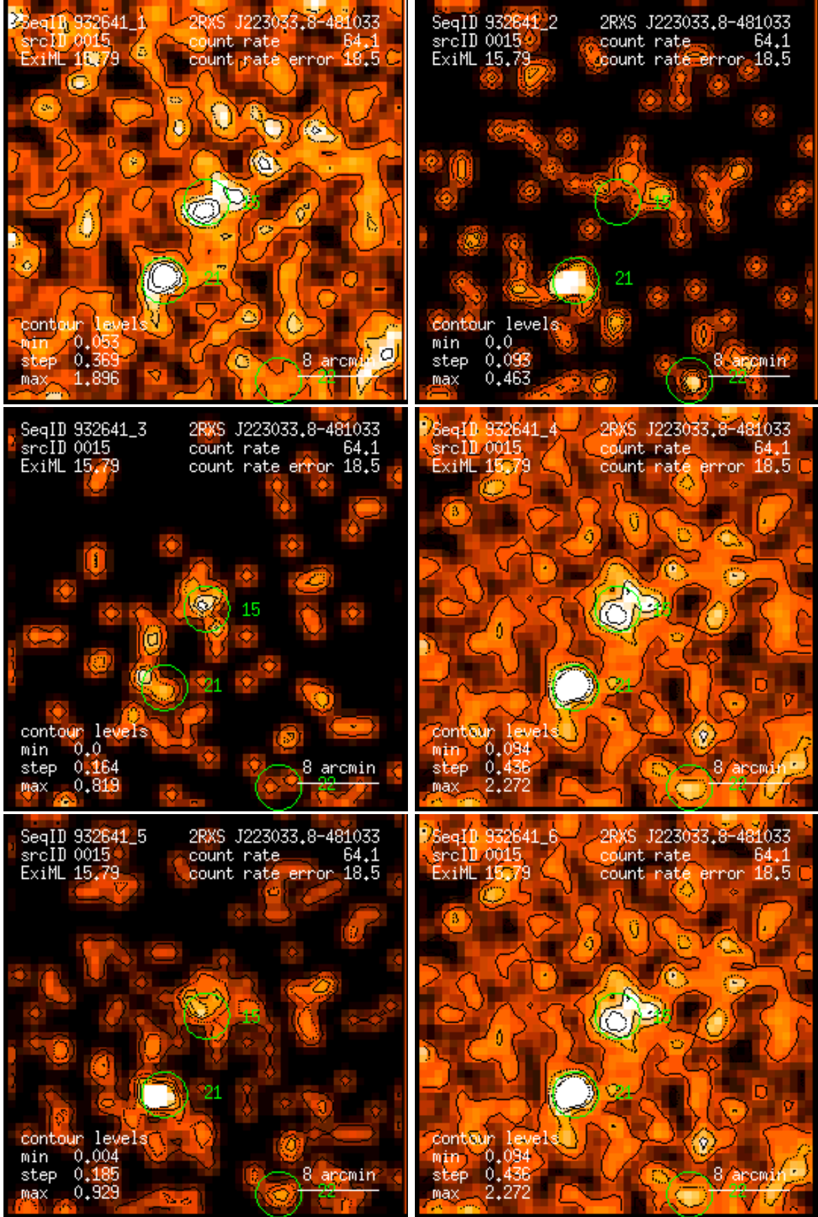
Figure 15: RASS 932641: detection 0015: band rate images, Gaussian filter: (1) PSPC channels 11 – 41, (2) 52 – 90, (3) 91 – 201, (4) 11 – 235, (5) 52 – 201, (6) 11 – 201. Broad band rates in counts/ks. Band rate contour levels in counts/ks/arcmin 2 .
