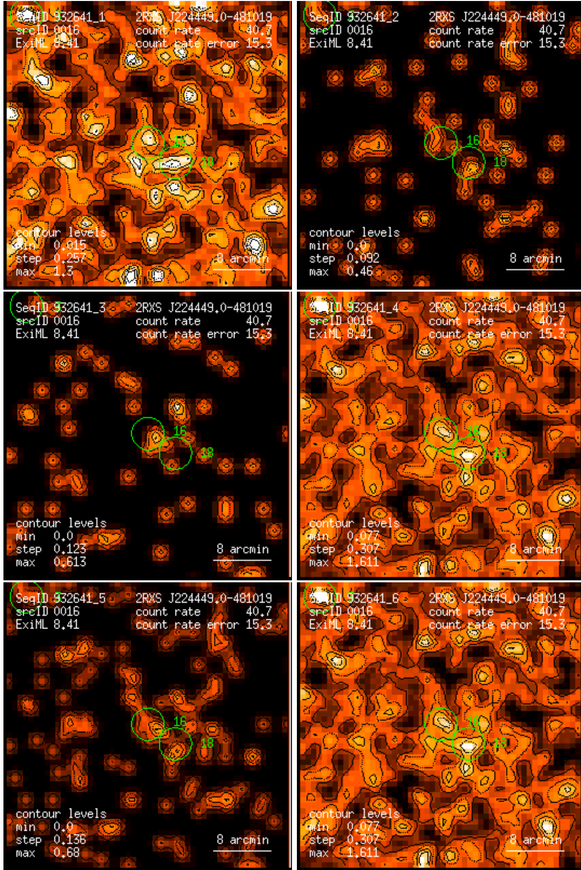
Figure 16: RASS 932641: detection 0016: band rate images, Gaussian filter: (1) PSPC channels 11 – 41, (2) 52 – 90, (3) 91 – 201, (4) 11 – 235, (5) 52 – 201, (6) 11 – 201. Broad band rates in counts/ks. Band rate contour levels in counts/ks/arcmin 2 .
