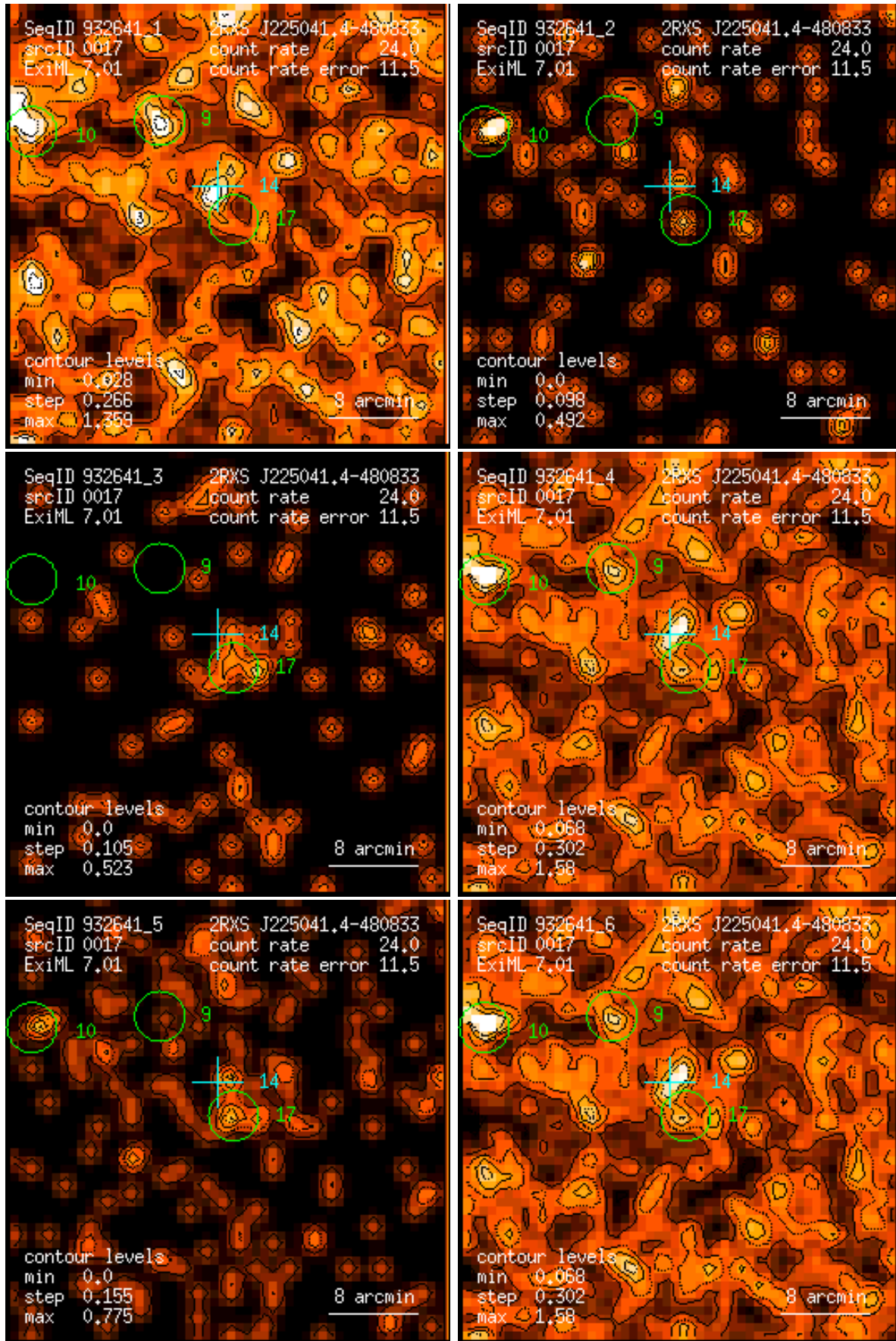
Figure 17: RASS 932641: detection 0017: band rate images, Gaussian filter: (1) PSPC channels 11 – 41, (2) 52 – 90, (3) 91 – 201, (4) 11 – 235, (5) 52 – 201, (6) 11 – 201. Broad band rates in counts/ks. Band rate contour levels in counts/ks/arcmin 2 .
