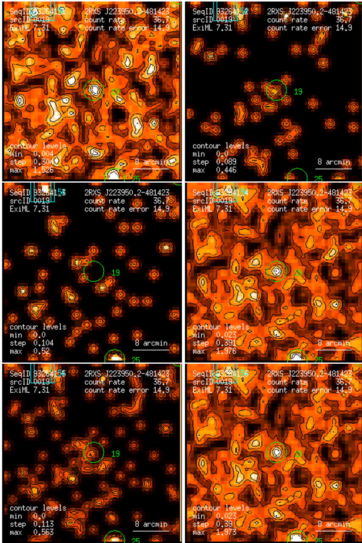
Figure 19: RASS 932641: detection 0019: band rate images, Gaussian filter: (1) PSPC channels 11 – 41, (2) 52 – 90, (3) 91 – 201, (4) 11 – 235, (5) 52 – 201, (6) 11 – 201. Broad band rates in counts/ks. Band rate contour levels in counts/ks/arcmin 2 .
