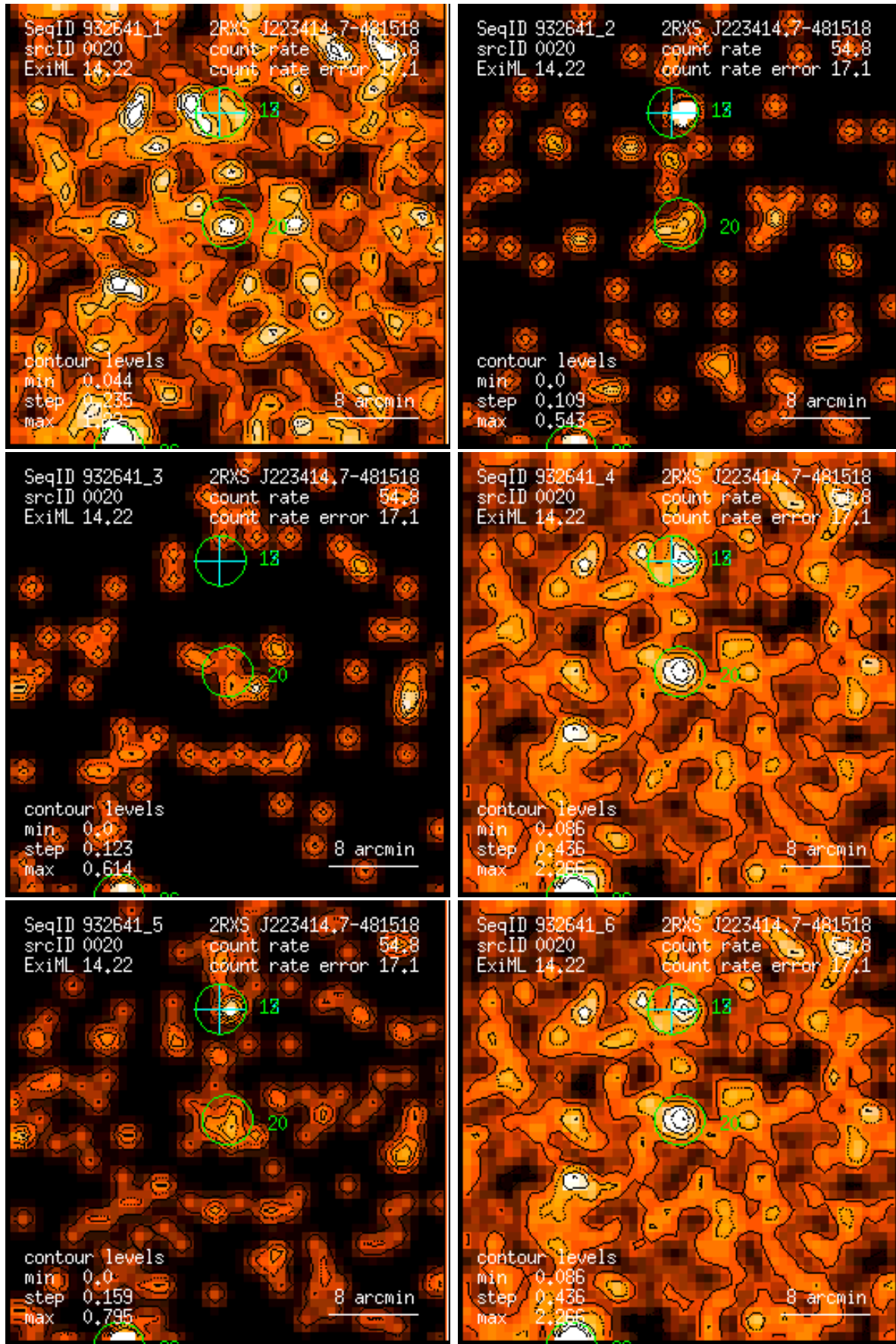
Figure 20: RASS 932641: detection 0020: band rate images, Gaussian filter: (1) PSPC channels 11 – 41, (2) 52 – 90, (3) 91 – 201, (4) 11 – 235, (5) 52 – 201, (6) 11 – 201. Broad band rates in counts/ks. Band rate contour levels in counts/ks/arcmin 2 .
