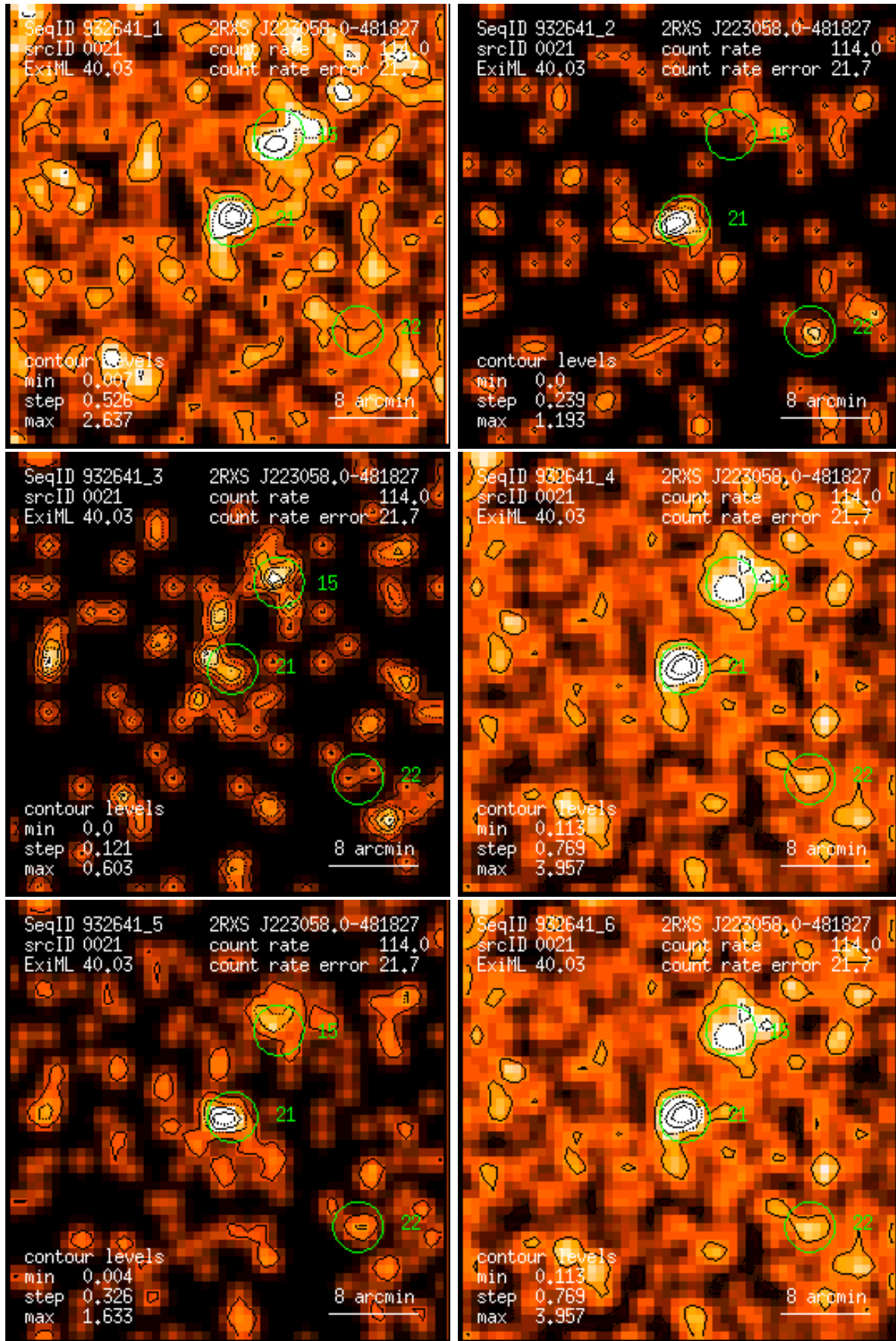
Figure 21: RASS 932641: detection 0021: band rate images, Gaussian filter: (1) PSPC channels 11 – 41, (2) 52 – 90, (3) 91 – 201, (4) 11 – 235, (5) 52 – 201, (6) 11 – 201. Broad band rates in counts/ks. Band rate contour levels in counts/ks/arcmin 2 .
