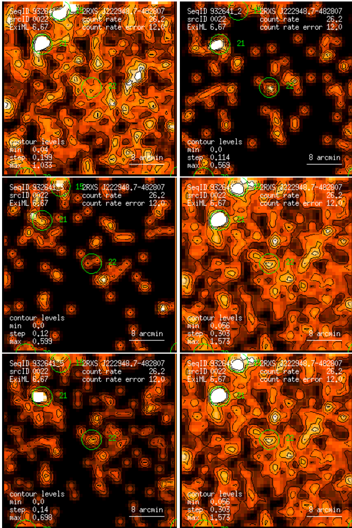
Figure 22: RASS 932641: detection 0022: band rate images, Gaussian filter: (1) PSPC channels 11 – 41, (2) 52 – 90, (3) 91 – 201, (4) 11 – 235, (5) 52 – 201, (6) 11 – 201. Broad band rates in counts/ks. Band rate contour levels in counts/ks/arcmin 2 .
