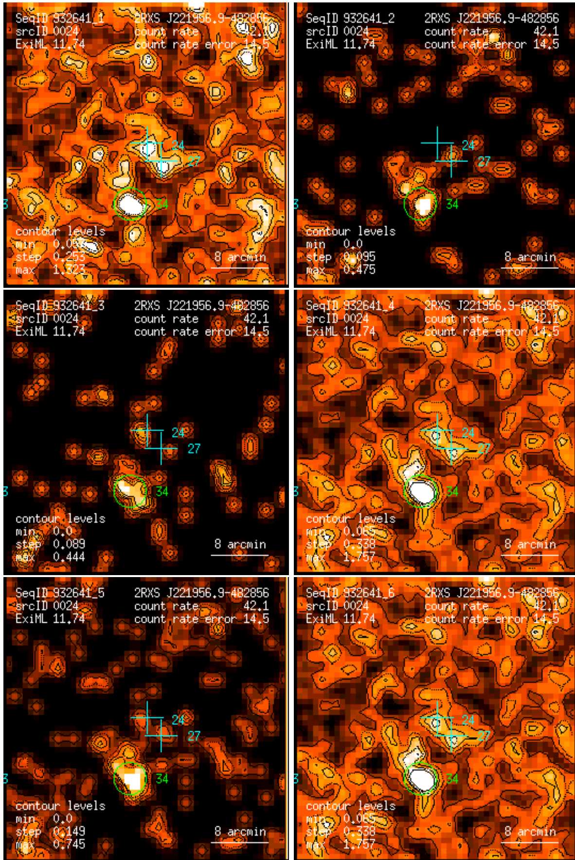
Figure 24: RASS 932641: detection 0024: band rate images, Gaussian filter: (1) PSPC channels 11 – 41, (2) 52 – 90, (3) 91 – 201, (4) 11 – 235, (5) 52 – 201, (6) 11 – 201. Broad band rates in counts/ks. Band rate contour levels in counts/ks/arcmin 2 .
