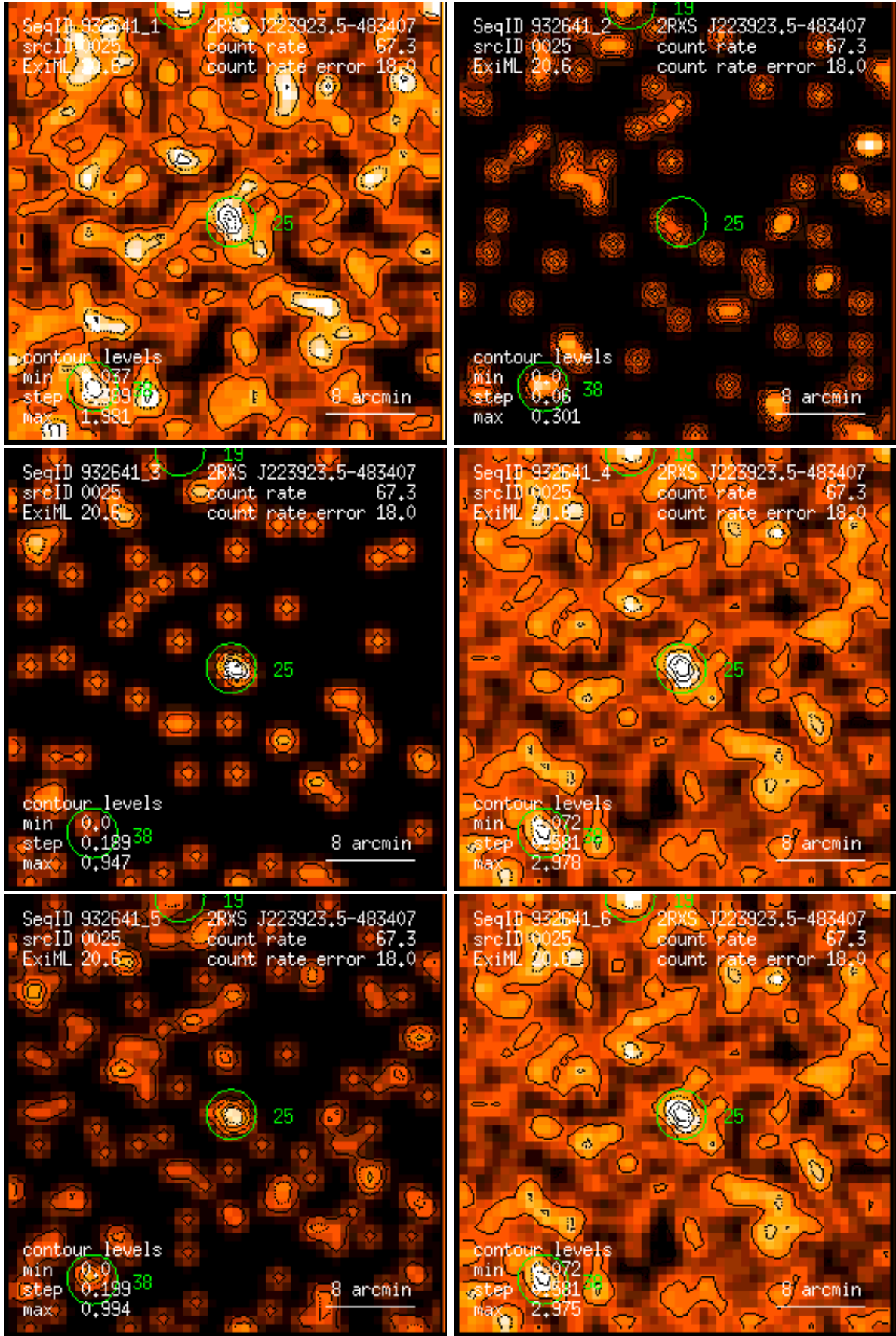
Figure 25: RASS 932641: detection 0025: band rate images, Gaussian filter: (1) PSPC channels 11 – 41, (2) 52 – 90, (3) 91 – 201, (4) 11 – 235, (5) 52 – 201, (6) 11 – 201. Broad band rates in counts/ks. Band rate contour levels in counts/ks/arcmin 2 .
