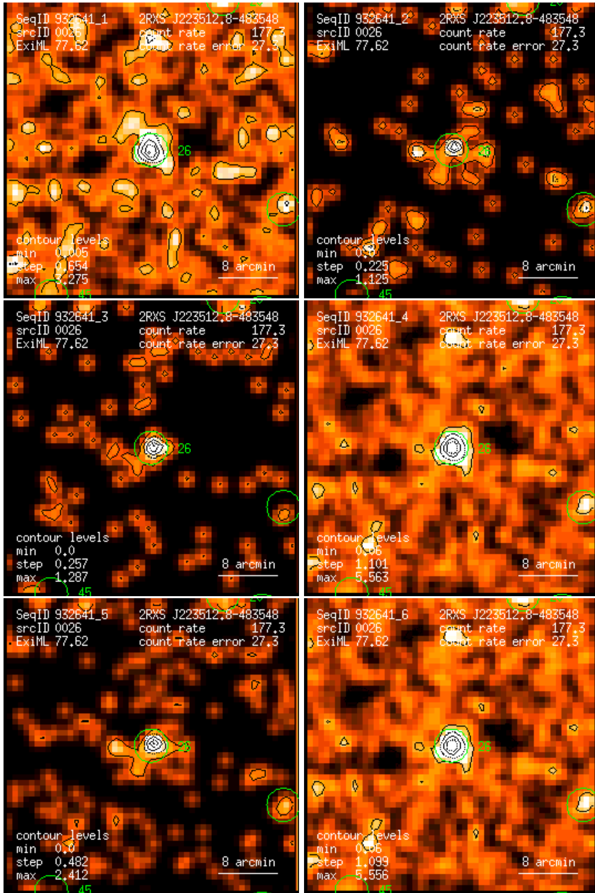
Figure 26: RASS 932641: detection 0026: band rate images, Gaussian filter: (1) PSPC channels 11 – 41, (2) 52 – 90, (3) 91 – 201, (4) 11 – 235, (5) 52 – 201, (6) 11 – 201. Broad band rates in counts/ks. Band rate contour levels in counts/ks/arcmin 2 .
