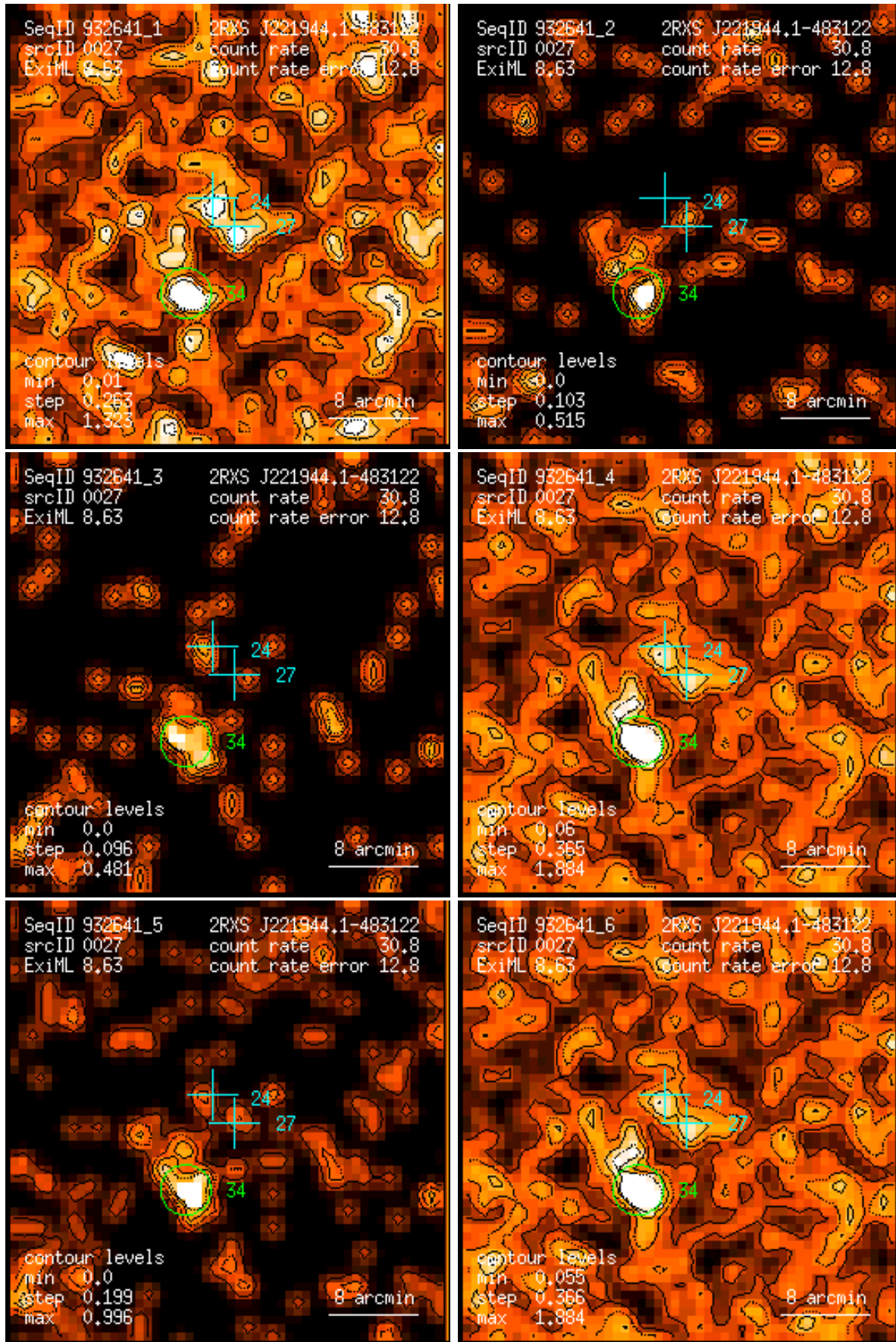
Figure 27: RASS 932641: detection 0027: band rate images, Gaussian filter: (1) PSPC channels 11 – 41, (2) 52 – 90, (3) 91 – 201, (4) 11 – 235, (5) 52 – 201, (6) 11 – 201. Broad band rates in counts/ks. Band rate contour levels in counts/ks/arcmin 2 .
