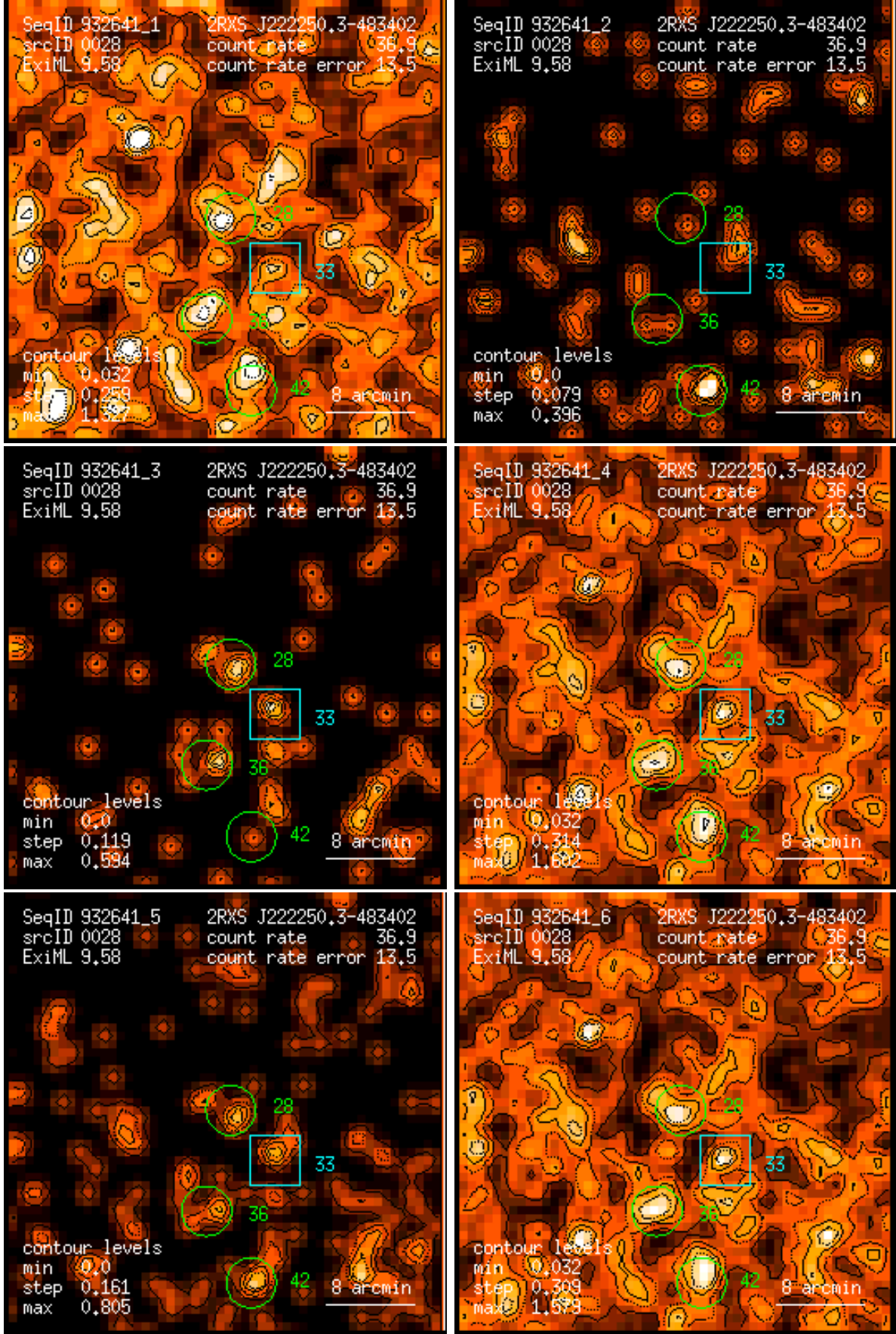
Figure 28: RASS 932641: detection 0028: band rate images, Gaussian filter: (1) PSPC channels 11 – 41, (2) 52 – 90, (3) 91 – 201, (4) 11 – 235, (5) 52 – 201, (6) 11 – 201. Broad band rates in counts/ks. Band rate contour levels in counts/ks/arcmin 2 .
