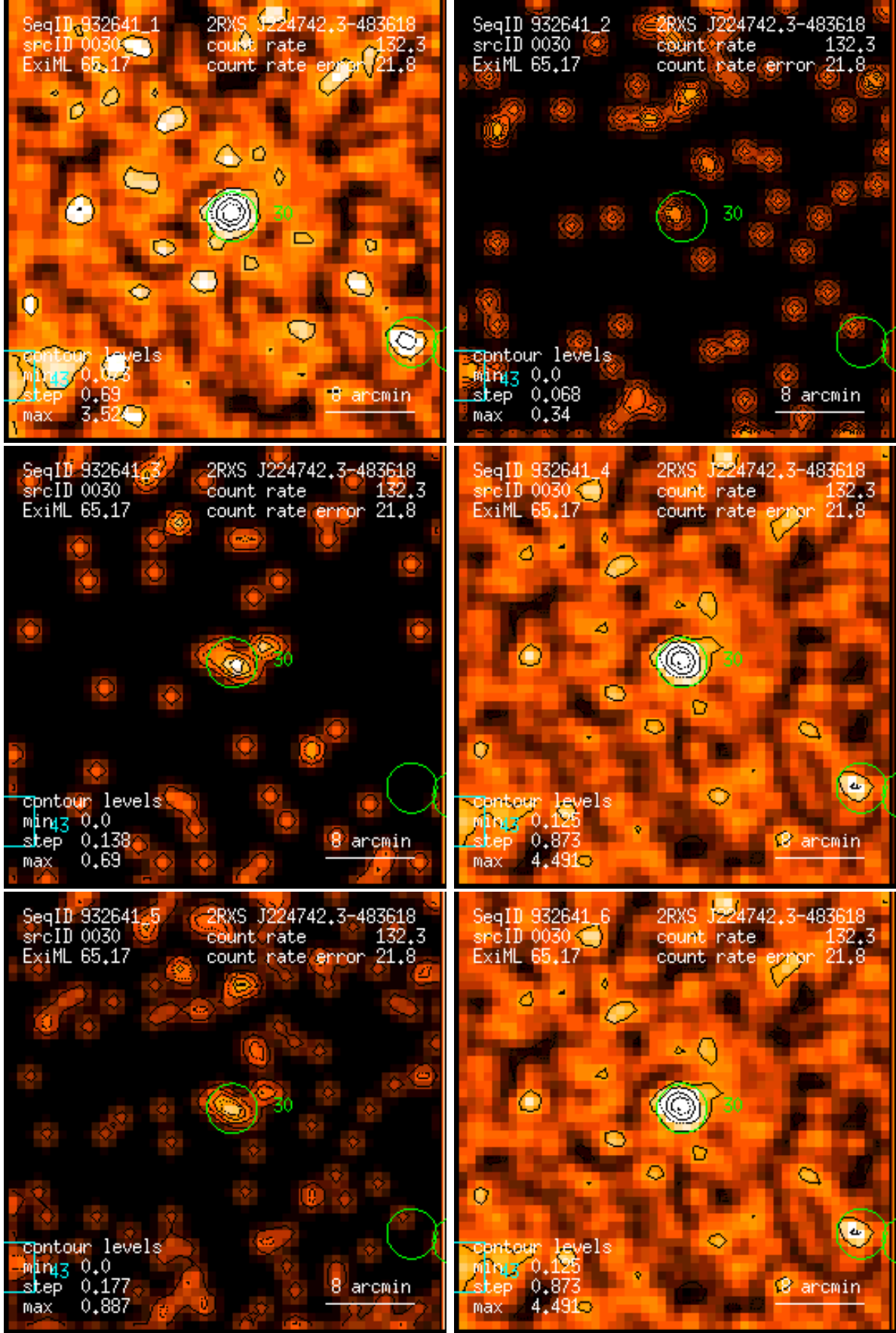
Figure 30: RASS 932641: detection 0030: band rate images, Gaussian filter: (1) PSPC channels 11 – 41, (2) 52 – 90, (3) 91 – 201, (4) 11 – 235, (5) 52 – 201, (6) 11 – 201. Broad band rates in counts/ks. Band rate contour levels in counts/ks/arcmin 2 .
