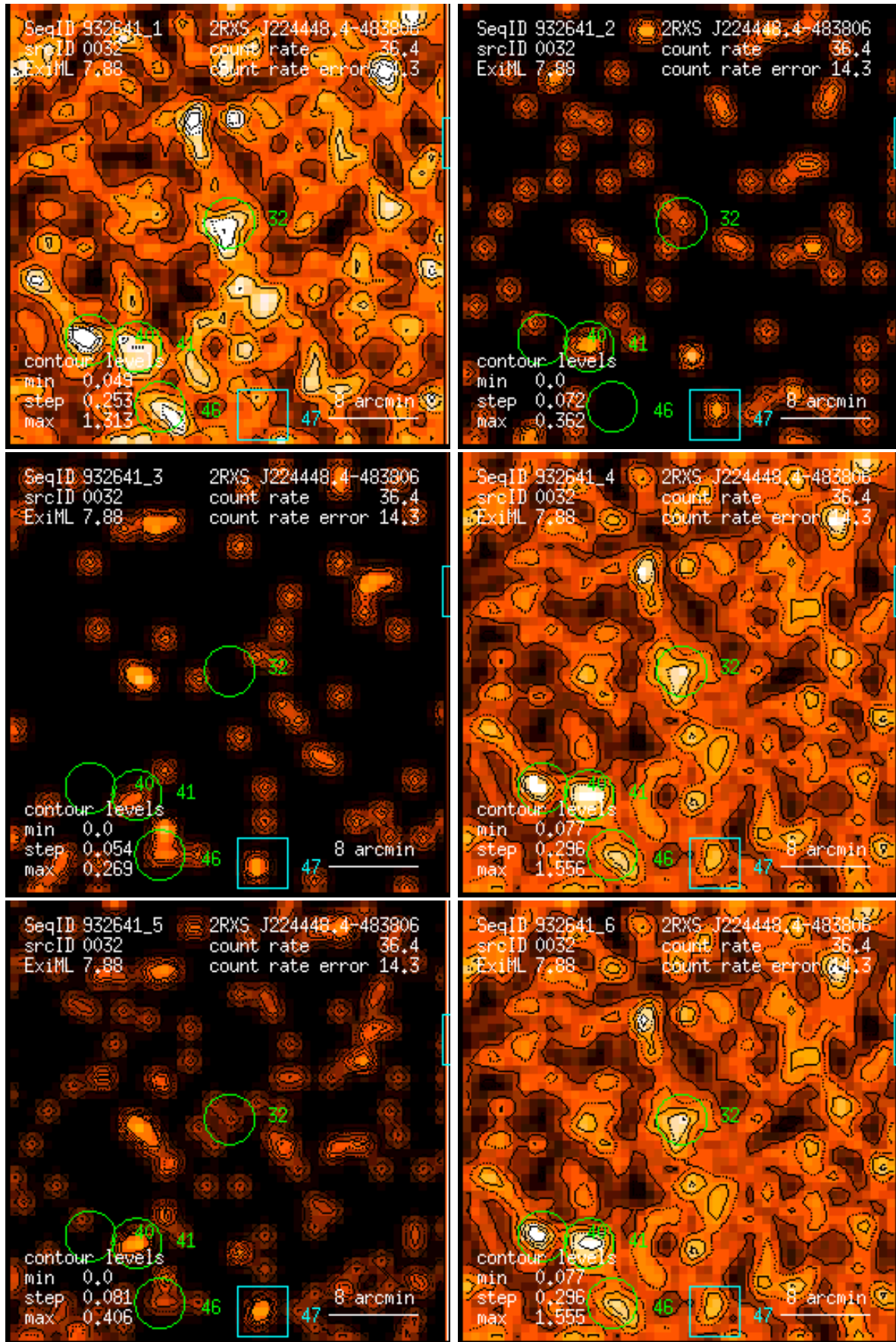
Figure 32: RASS 932641: detection 0032: band rate images, Gaussian filter: (1) PSPC channels 11 – 41, (2) 52 – 90, (3) 91 – 201, (4) 11 – 235, (5) 52 – 201, (6) 11 – 201. Broad band rates in counts/ks. Band rate contour levels in counts/ks/arcmin 2 .
