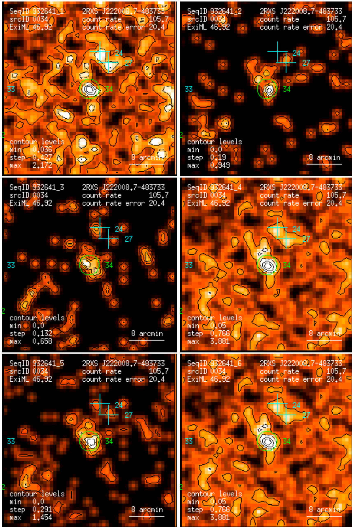
Figure 34: RASS 932641: detection 0034: band rate images, Gaussian filter: (1) PSPC channels 11 – 41, (2) 52 – 90, (3) 91 – 201, (4) 11 – 235, (5) 52 – 201, (6) 11 – 201. Broad band rates in counts/ks. Band rate contour levels in counts/ks/arcmin 2 .
