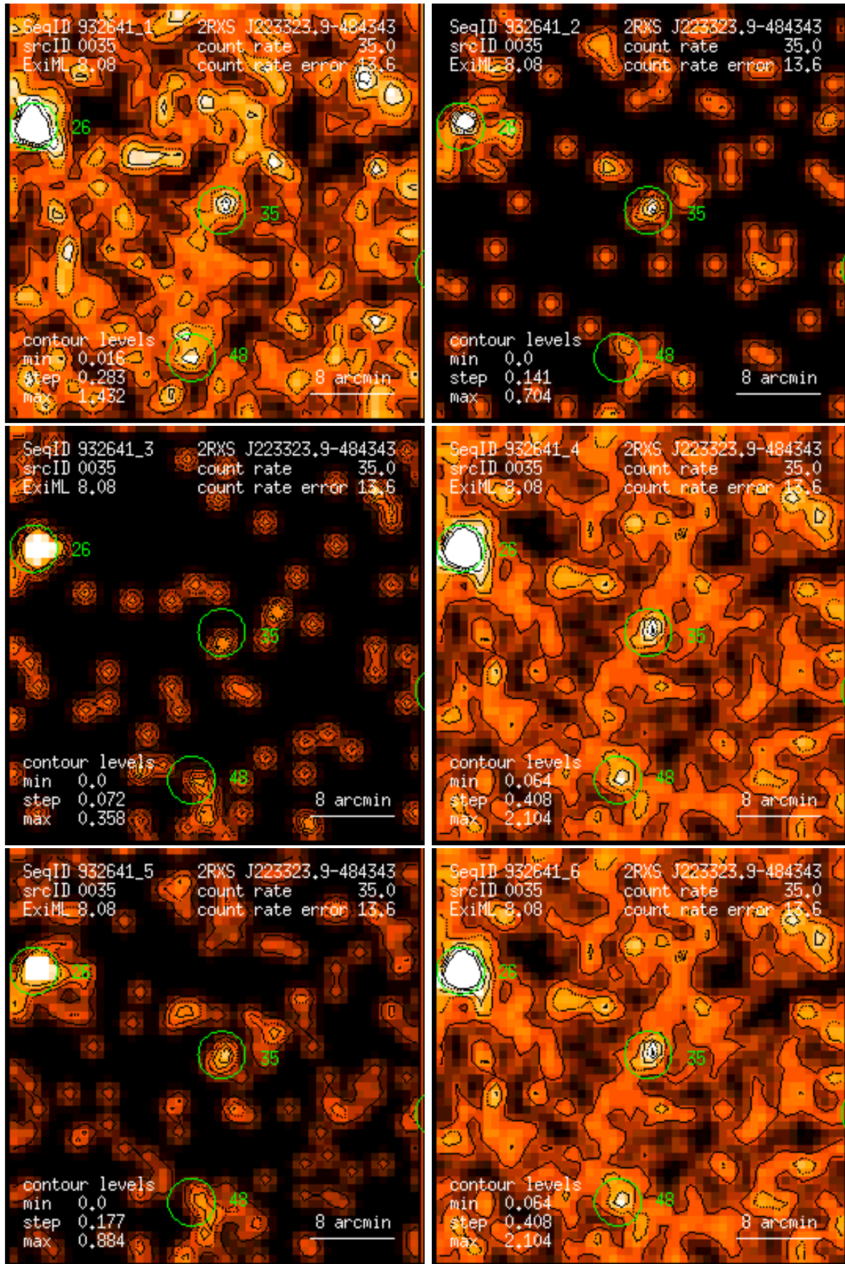
Figure 35: RASS 932641: detection 0035: band rate images, Gaussian filter: (1) PSPC channels 11 – 41, (2) 52 – 90, (3) 91 – 201, (4) 11 – 235, (5) 52 – 201, (6) 11 – 201. Broad band rates in counts/ks. Band rate contour levels in counts/ks/arcmin 2 .
