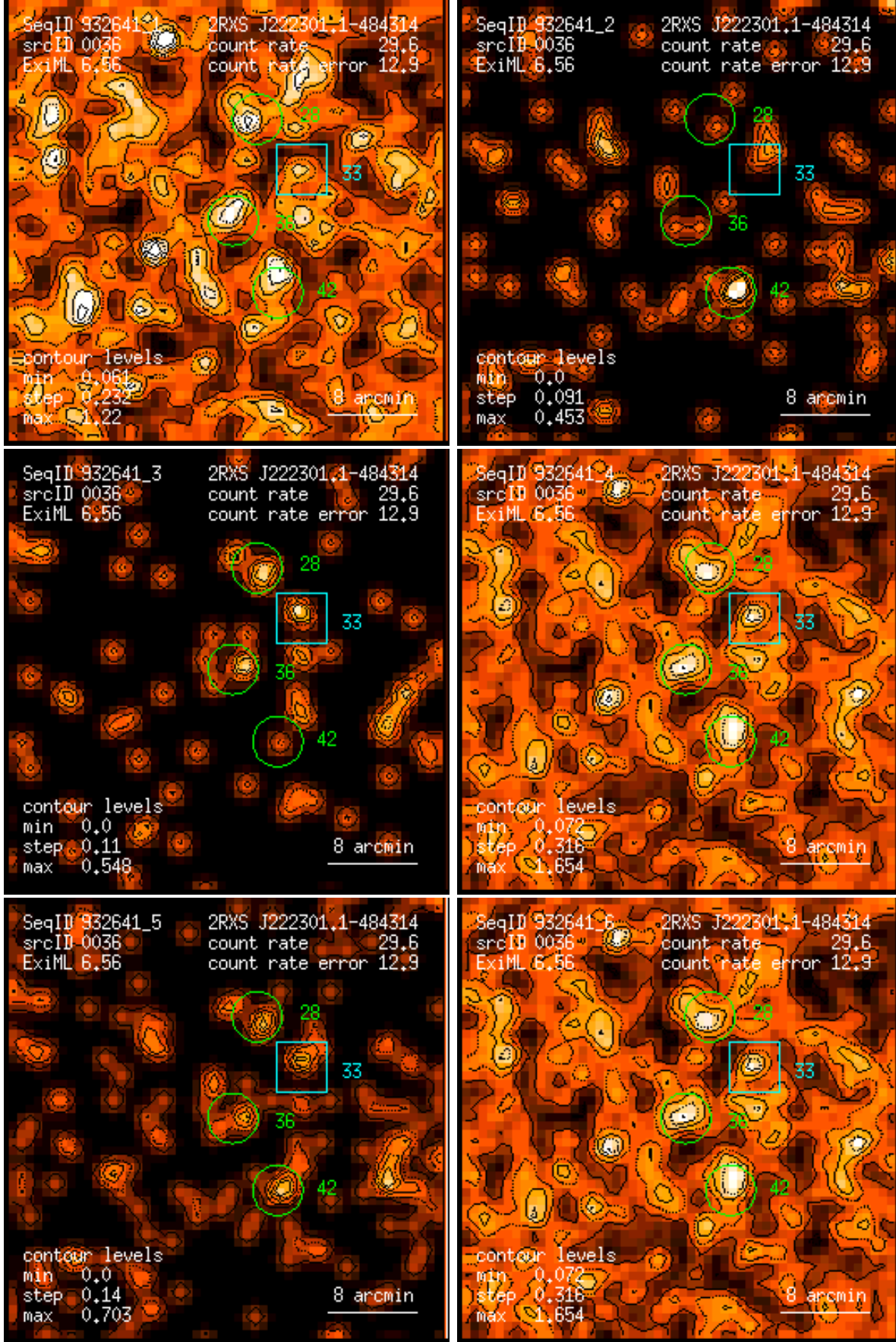
Figure 36: RASS 932641: detection 0036: band rate images, Gaussian filter: (1) PSPC channels 11 – 41, (2) 52 – 90, (3) 91 – 201, (4) 11 – 235, (5) 52 – 201, (6) 11 – 201. Broad band rates in counts/ks. Band rate contour levels in counts/ks/arcmin 2 .
