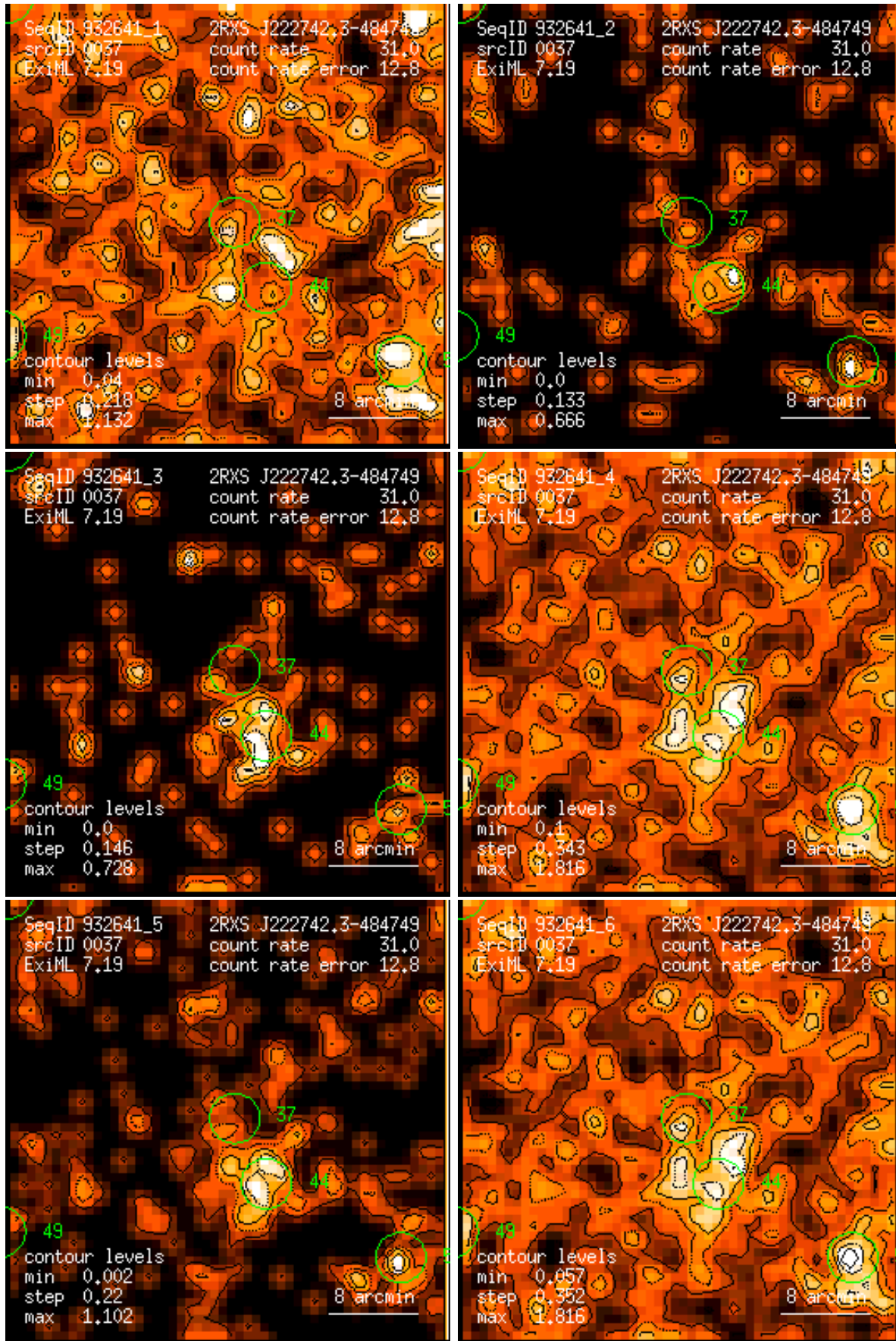
Figure 37: RASS 932641: detection 0037: band rate images, Gaussian filter: (1) PSPC channels 11 – 41, (2) 52 – 90, (3) 91 – 201, (4) 11 – 235, (5) 52 – 201, (6) 11 – 201. Broad band rates in counts/ks. Band rate contour levels in counts/ks/arcmin 2 .
