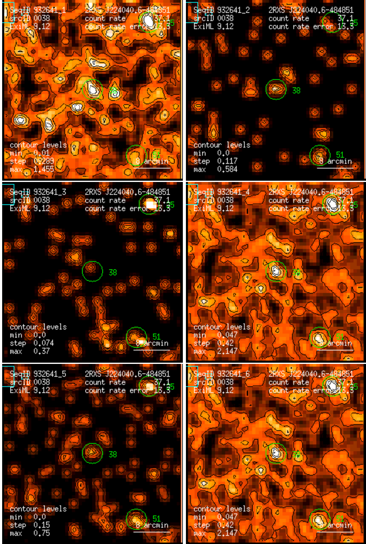
Figure 38: RASS 932641: detection 0038: band rate images, Gaussian filter: (1) PSPC channels 11 – 41, (2) 52 – 90, (3) 91 – 201, (4) 11 – 235, (5) 52 – 201, (6) 11 – 201. Broad band rates in counts/ks. Band rate contour levels in counts/ks/arcmin 2 .
