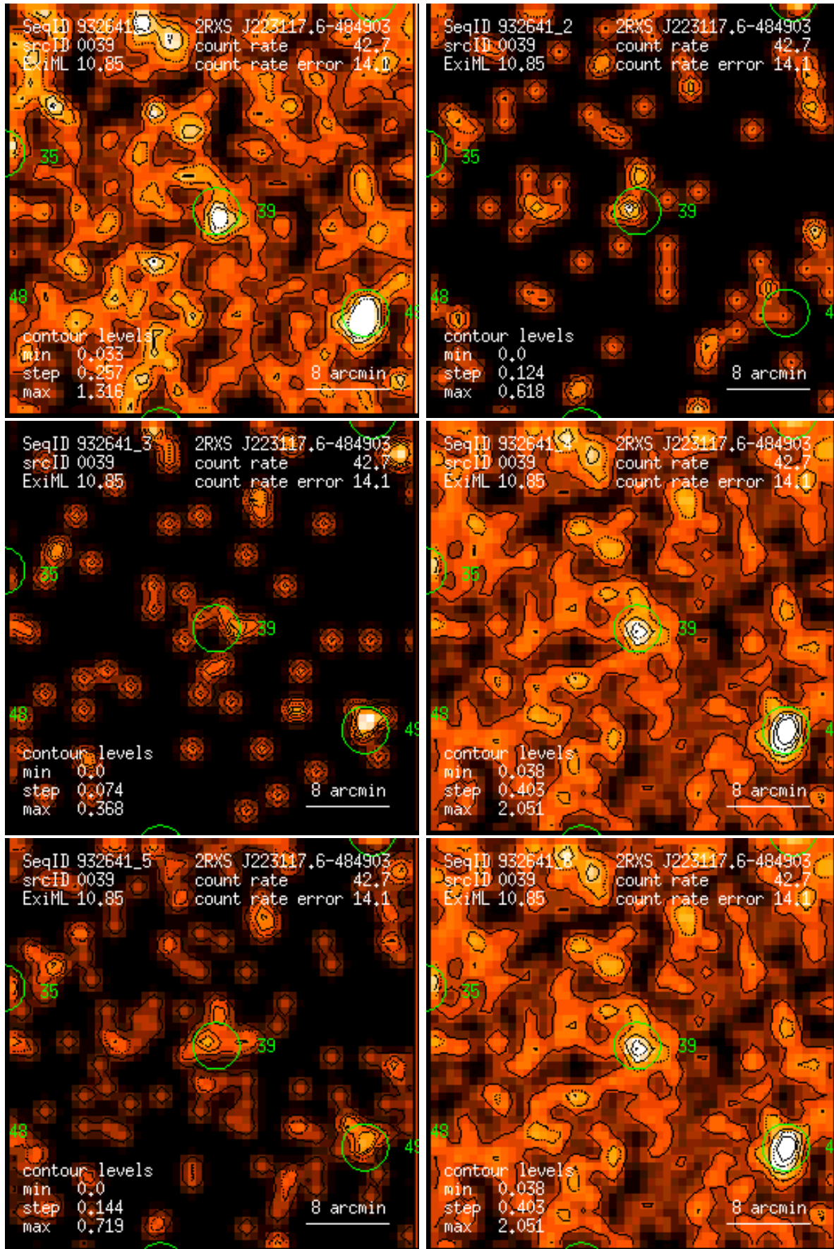
Figure 39: RASS 932641: detection 0039: band rate images, Gaussian filter: (1) PSPC channels 11 – 41, (2) 52 – 90, (3) 91 – 201, (4) 11 – 235, (5) 52 – 201, (6) 11 – 201. Broad band rates in counts/ks. Band rate contour levels in counts/ks/arcmin 2 .
