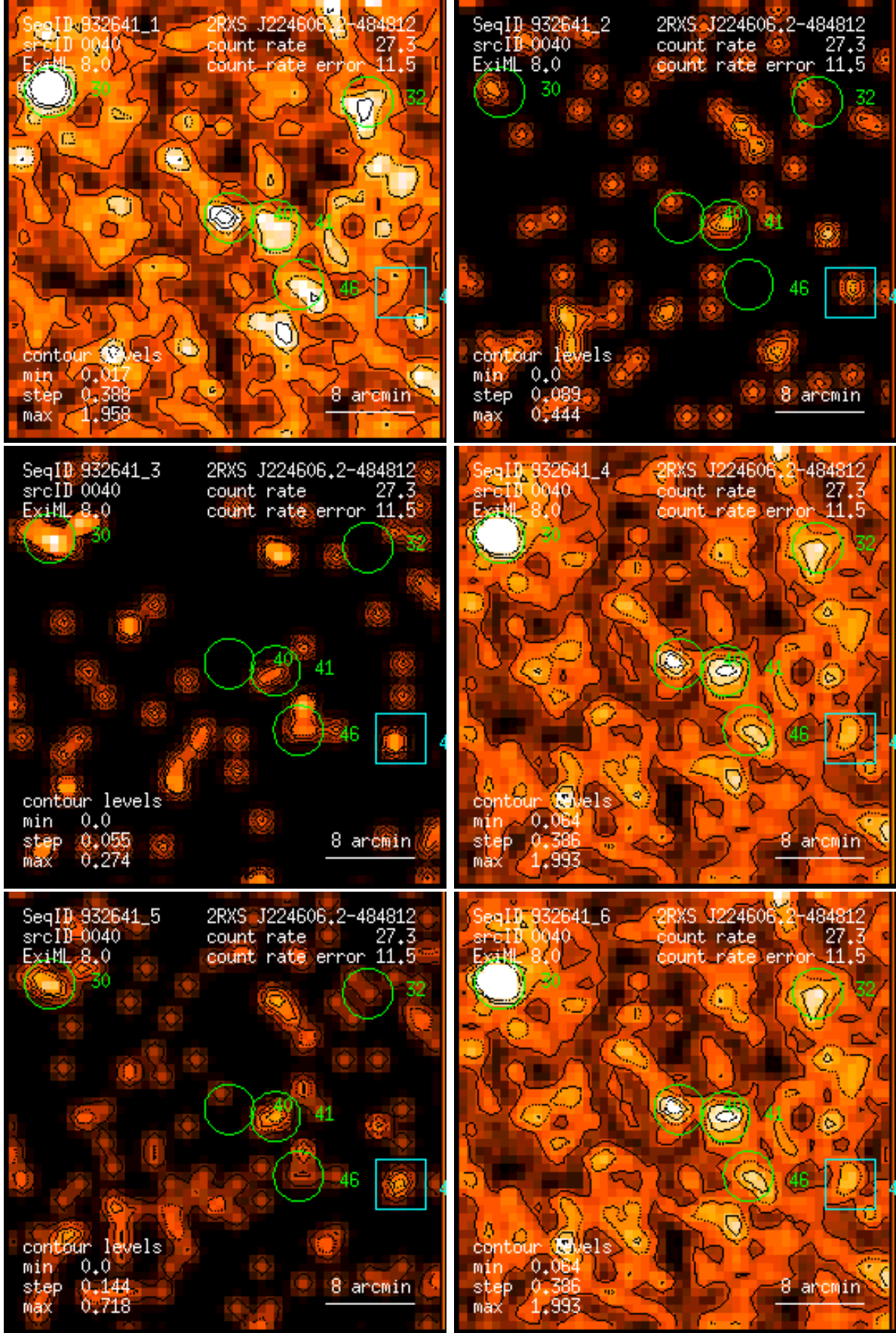
Figure 40: RASS 932641: detection 0040: band rate images, Gaussian filter: (1) PSPC channels 11 – 41, (2) 52 – 90, (3) 91 – 201, (4) 11 – 235, (5) 52 – 201, (6) 11 – 201. Broad band rates in counts/ks. Band rate contour levels in counts/ks/arcmin 2 .
