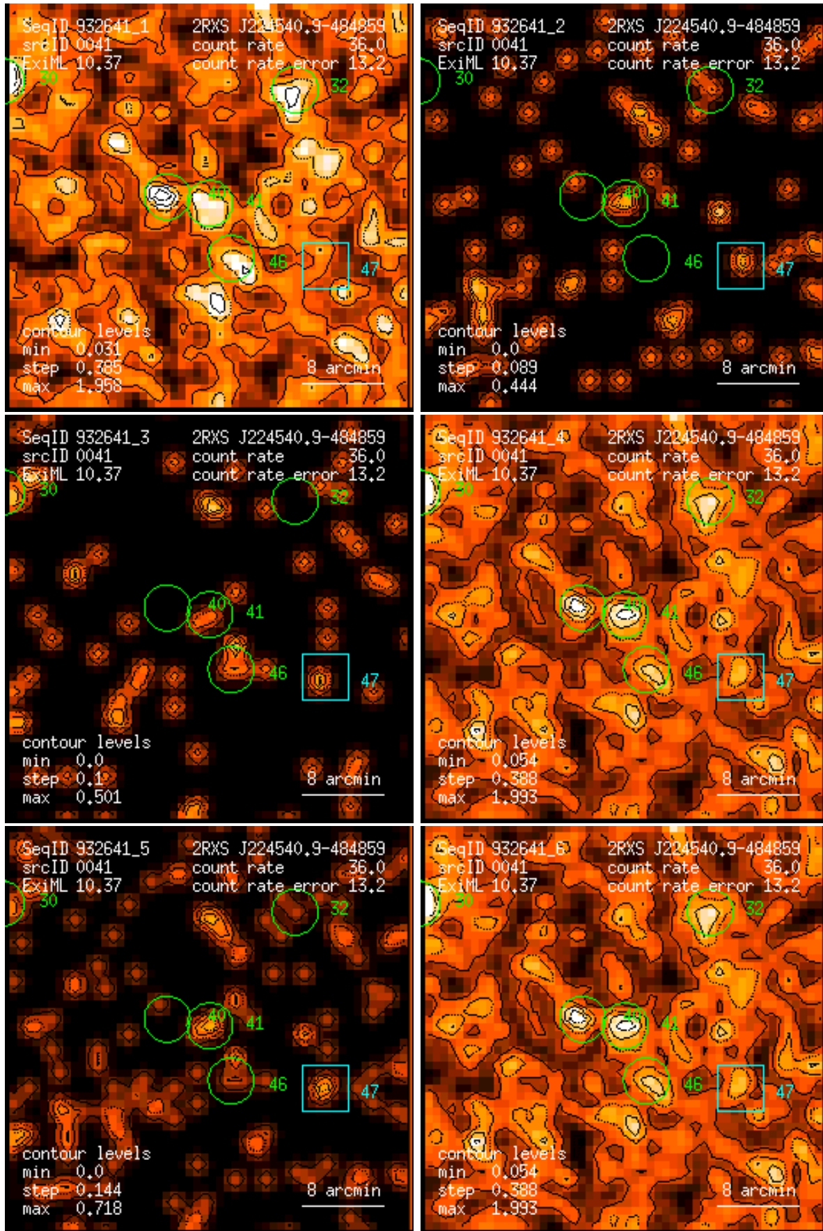
Figure 41: RASS 932641: detection 0041: band rate images, Gaussian filter: (1) PSPC channels 11 – 41, (2) 52 – 90, (3) 91 – 201, (4) 11 – 235, (5) 52 – 201, (6) 11 – 201. Broad band rates in counts/ks. Band rate contour levels in counts/ks/arcmin 2 .
