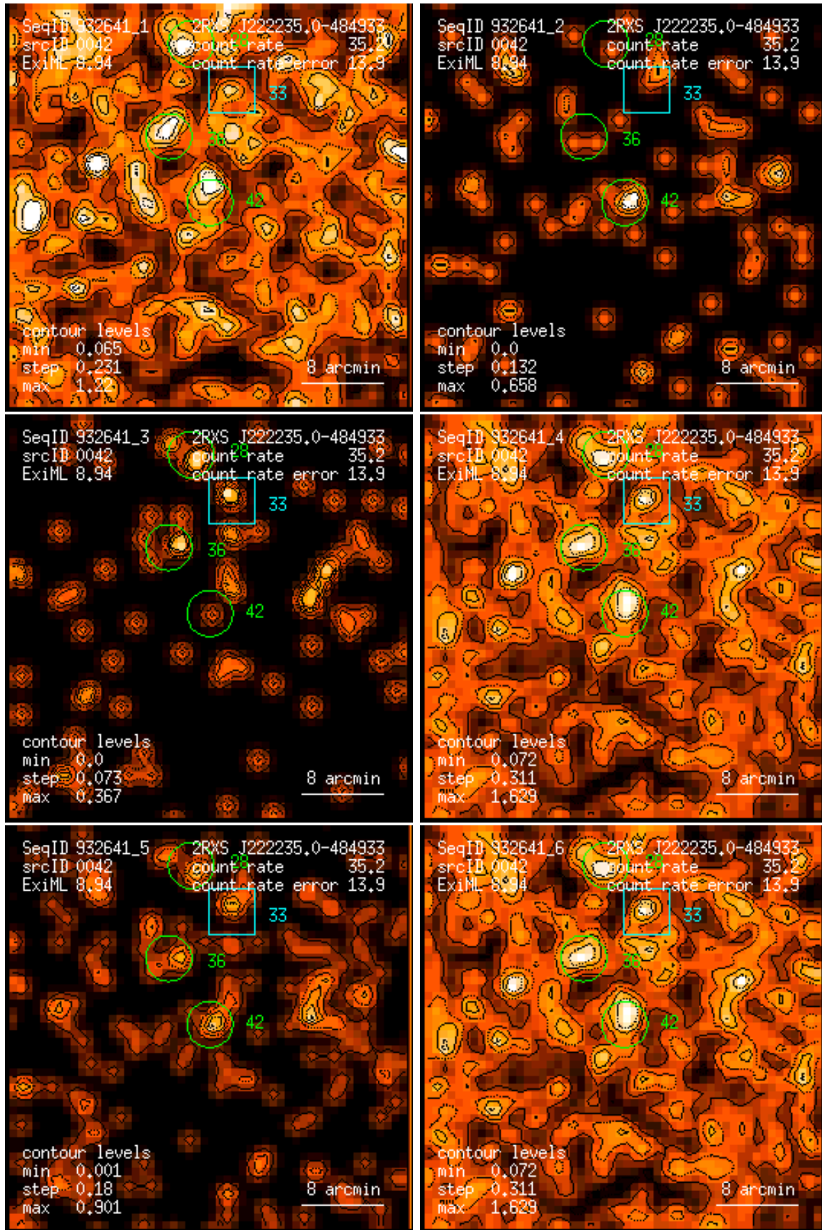
Figure 42: RASS 932641: detection 0042: band rate images, Gaussian filter: (1) PSPC channels 11 – 41, (2) 52 – 90, (3) 91 – 201, (4) 11 – 235, (5) 52 – 201, (6) 11 – 201. Broad band rates in counts/ks. Band rate contour levels in counts/ks/arcmin 2 .
