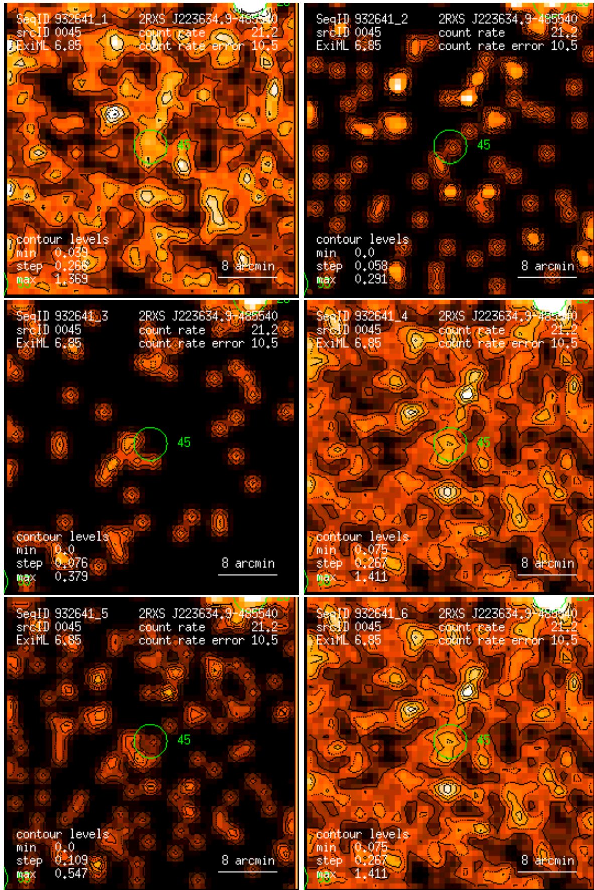
Figure 45: RASS 932641: detection 0045: band rate images, Gaussian filter: (1) PSPC channels 11 – 41, (2) 52 – 90, (3) 91 – 201, (4) 11 – 235, (5) 52 – 201, (6) 11 – 201. Broad band rates in counts/ks. Band rate contour levels in counts/ks/arcmin 2 .
