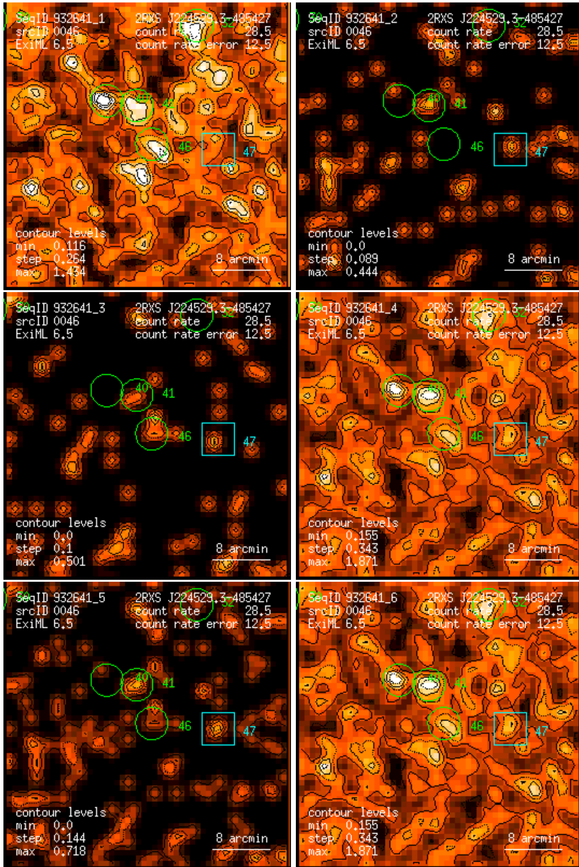
Figure 46: RASS 932641: detection 0046: band rate images, Gaussian filter: (1) PSPC channels 11 – 41, (2) 52 – 90, (3) 91 – 201, (4) 11 – 235, (5) 52 – 201, (6) 11 – 201. Broad band rates in counts/ks. Band rate contour levels in counts/ks/arcmin 2 .
