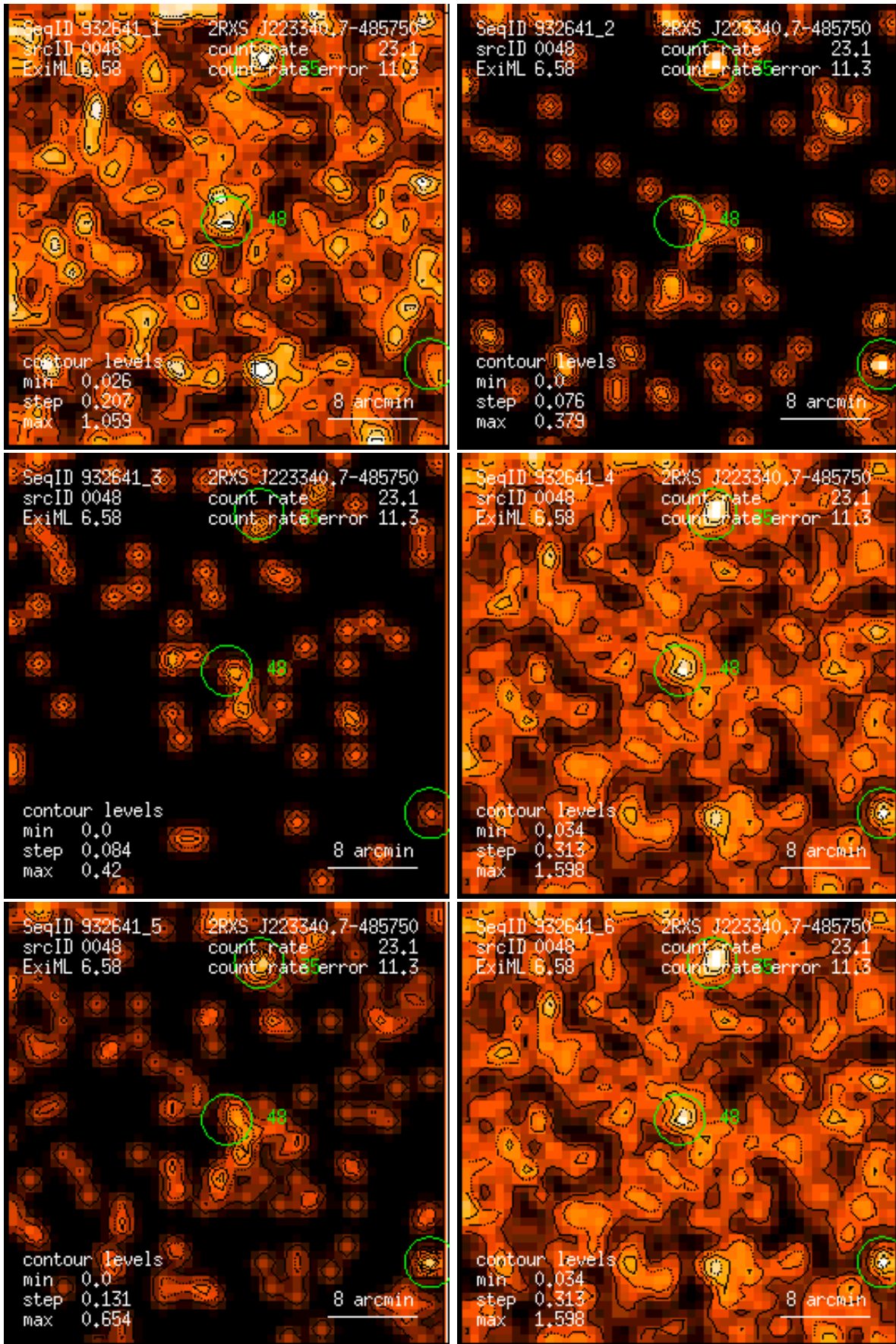
Figure 48: RASS 932641: detection 0048: band rate images, Gaussian filter: (1) PSPC channels 11 – 41, (2) 52 – 90, (3) 91 – 201, (4) 11 – 235, (5) 52 – 201, (6) 11 – 201. Broad band rates in counts/ks. Band rate contour levels in counts/ks/arcmin 2 .
