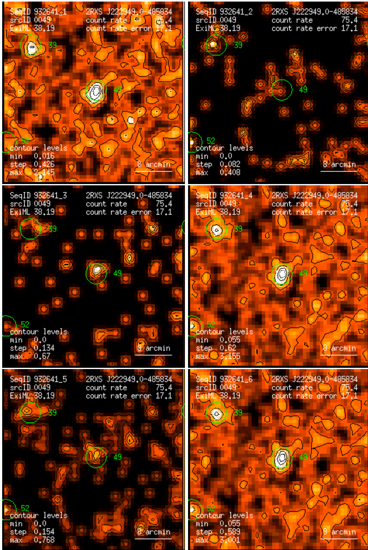
Figure 49: RASS 932641: detection 0049: band rate images, Gaussian filter: (1) PSPC channels 11 – 41, (2) 52 – 90, (3) 91 – 201, (4) 11 – 235, (5) 52 – 201, (6) 11 – 201. Broad band rates in counts/ks. Band rate contour levels in counts/ks/arcmin 2 .
