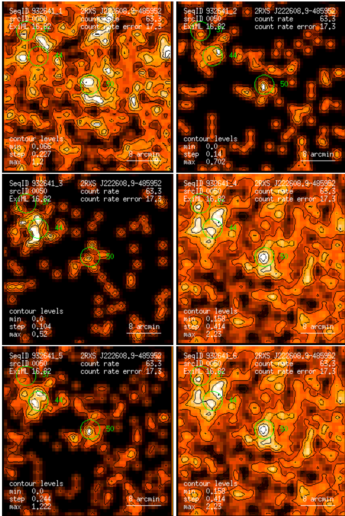
Figure 50: RASS 932641: detection 0050: band rate images, Gaussian filter: (1) PSPC channels 11 – 41, (2) 52 – 90, (3) 91 – 201, (4) 11 – 235, (5) 52 – 201, (6) 11 – 201. Broad band rates in counts/ks. Band rate contour levels in counts/ks/arcmin 2 .
