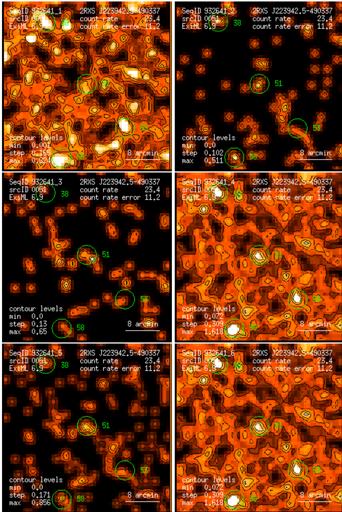
Figure 51: RASS 932641: detection 0051: band rate images, Gaussian filter: (1) PSPC channels 11 – 41, (2) 52 – 90, (3) 91 – 201, (4) 11 – 235, (5) 52 – 201, (6) 11 – 201. Broad band rates in counts/ks. Band rate contour levels in counts/ks/arcmin 2 .
