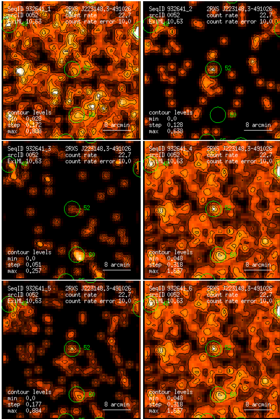
Figure 52: RASS 932641: detection 0052: band rate images, Gaussian filter: (1) PSPC channels 11 – 41, (2) 52 – 90, (3) 91 – 201, (4) 11 – 235, (5) 52 – 201, (6) 11 – 201. Broad band rates in counts/ks. Band rate contour levels in counts/ks/arcmin 2 .
