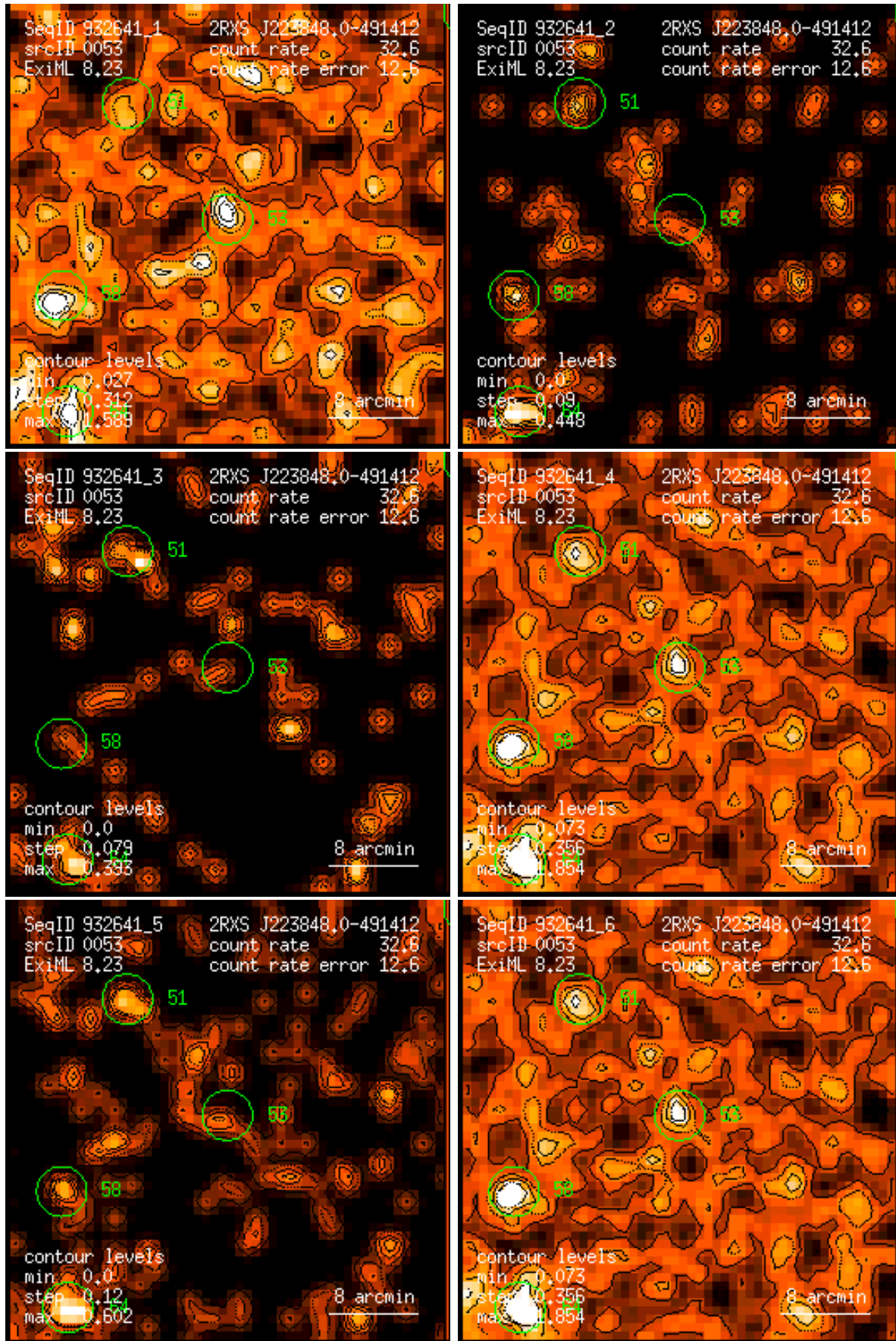
Figure 53: RASS 932641: detection 0053: band rate images, Gaussian filter: (1) PSPC channels 11 – 41, (2) 52 – 90, (3) 91 – 201, (4) 11 – 235, (5) 52 – 201, (6) 11 – 201. Broad band rates in counts/ks. Band rate contour levels in counts/ks/arcmin 2 .
