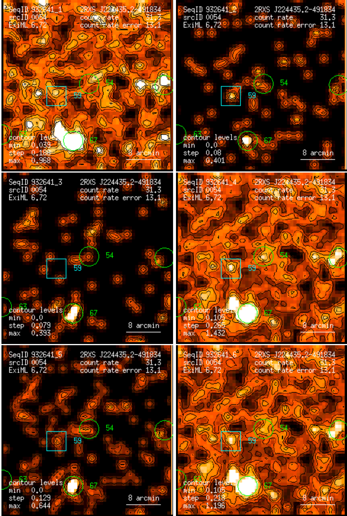
Figure 54: RASS 932641: detection 0054: band rate images, Gaussian filter: (1) PSPC channels 11 – 41, (2) 52 – 90, (3) 91 – 201, (4) 11 – 235, (5) 52 – 201, (6) 11 – 201. Broad band rates in counts/ks. Band rate contour levels in counts/ks/arcmin 2 .
